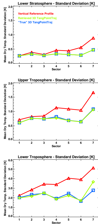
Fig. 6. Mean dry temperature standard deviation in the lower stratosphere between 20 km and 25 km altitude (top), in the upper troposphere between 5 km and 10 km (middle), and in the lower troposphere below 5 km (bottom; note the different y-axis range).
