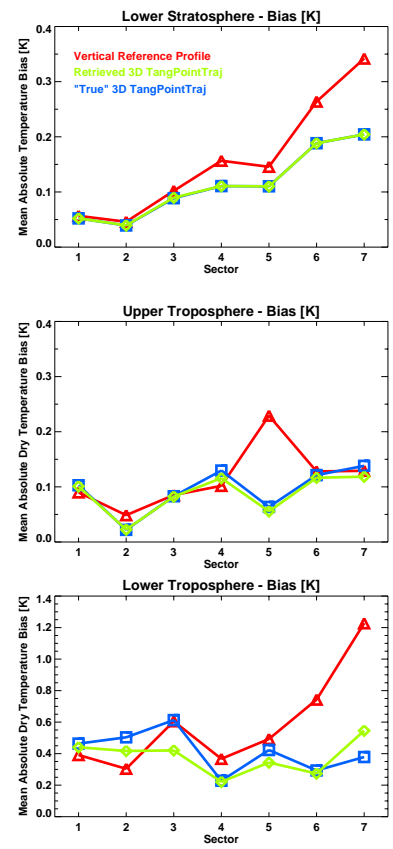
Fig. 7. Mean absolute dry temperature bias in the lower stratosphere between 20 km and 25 km altitude (top), in the upper troposphere between 5 km and 10 km (middle), and in the lower troposphere below 5 km (bottom; note the different y-axis range).
