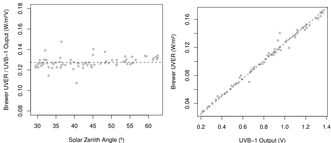
Fig. 2. Left: The ratio between the erythemally integrated irradiance given by the Brewer spectroradiometer and the YES UVB-1 radiometer output voltage as a function of the solar zenith angle during the Arenosillo's campaign 2007. The horizontal line represents the mean ratio ( 0.1275 \text{ Wm}^{-2}/\text{V} ). Right: Relationship between the Brewer erythemally integrated irradiance and the UVB-1 output voltage for SZA smaller than 65^\circ together with the regression line corresponding to the first-order model.
