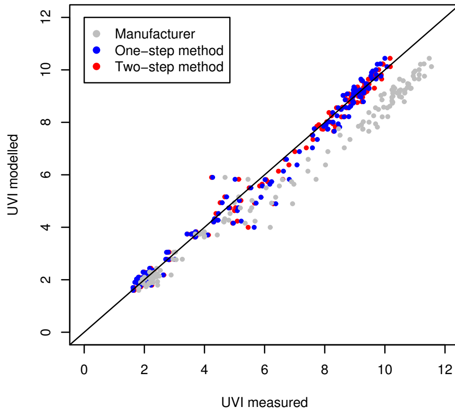
Fig. 5. Relationship between UVI estimations derived from LibRadtran/UVSPEC model and experimental UVI data obtained applying the manufacture’s factor and the two calibration procedures. The solid line is the zero bias line, unit slope.
