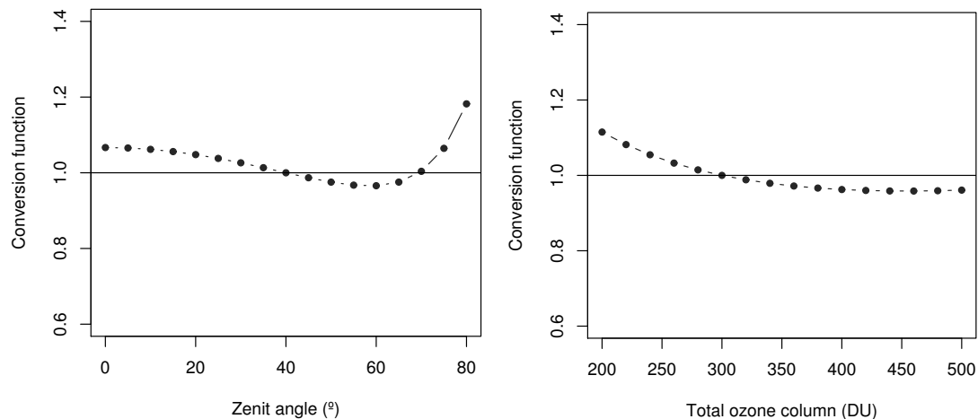
Fig. 3. Left: Variation of the normalized conversion function with respect to the solar zenith angle, for a constant total ozone column of 300 DU. Right: Variation of the normalized conversion function with respect to the total ozone column, for a constant solar zenith angle of 40^\circ .
