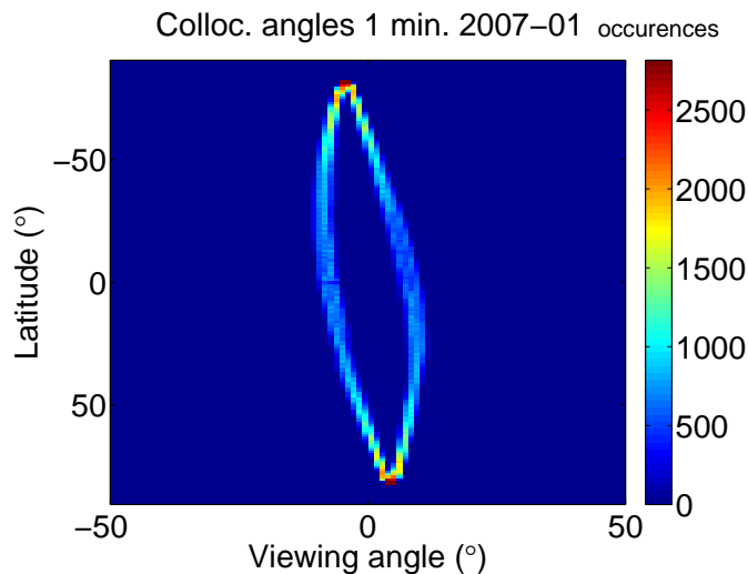
Fig. 3. This two-dimensional histogram shows at which angles the collocations between the NOAA-18 MHS and the CloudSat CPR occurred in January 2007. The figure shows collocations with a maximum time interval of 1 min.
