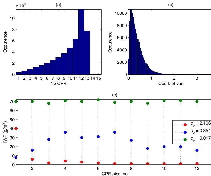
Fig. 5. Some collocation properties for 2007. (a) shows a histogram of the number of CPR pixels that fit inside a MHS pixel (circular with a 7.5 km radius). (b) shows a histogram for the coefficient of variation of the all collocations that contain only cloudy pixels. (c) shows examples of how CPR IWP may be distributed inside a MHS pixel. See text for a discussion.
