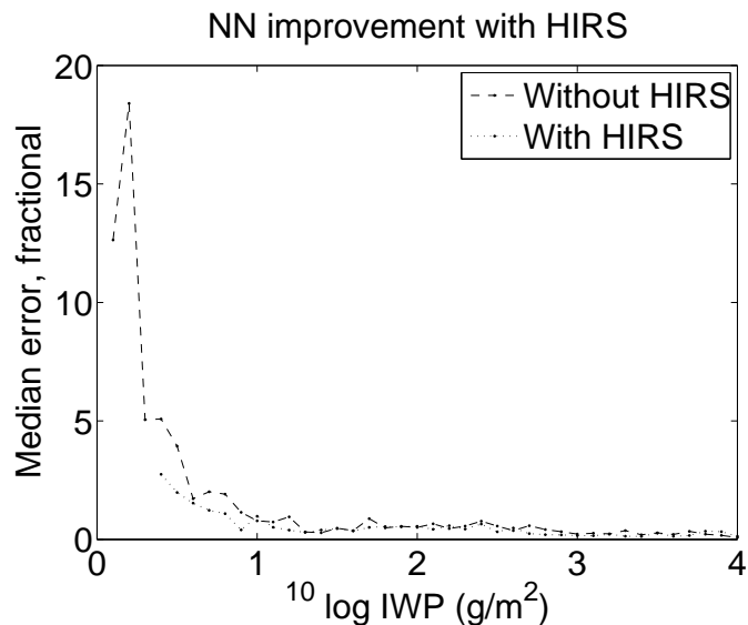
Fig. 12. Comparison of the median fractional error with and without adding the HIRS channels. The median fractional error is defined as the median of all errors with a certain IWP, where the error is defined as \left| \frac{\text{IWP}_{\text{NN}} - \text{IWP}_{\text{CPR}}}{\text{IWP}_{\text{CPR}}} \right| .
