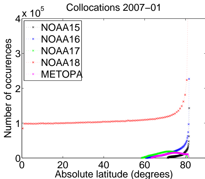
Fig. 2. A histogram of the number of collocations between the CloudSat CPR and the AMSU-B or MHS sensors on various satellites in January 2007. The maximum distance for a collocation is 15 km; the maximum time between the collocated measurements is 15 min (900 s). The number of collocations refers to the number of CloudSat pixels collocating with an AMSU-B or MHS pixel.
