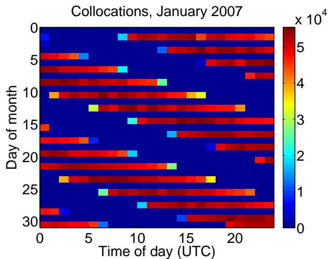
Fig. 4. Number of collocations in January 2007. The vertical axis shows the day of the month. The horizontal axis shows the universal time.
