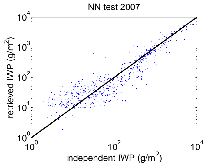
Fig. 9. Scatter plot to show the performance of the neural network, MHS 3–5.
