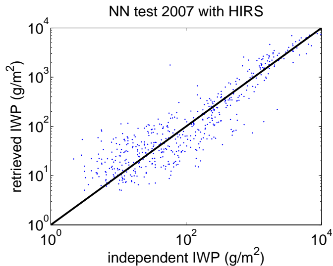
Fig. 11. Scatter plot to show the performance of the neural network, MHS 3–5, HIRS 8 and 11.
