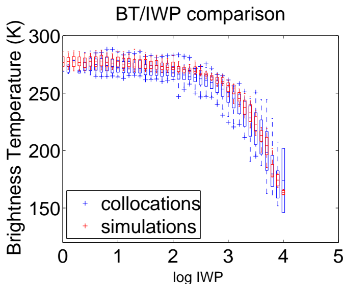
Fig. 7. Modified boxplot of Ice Water Path and MHS channel 5 or AMSU-B channel 20 brightness temperature. The horizontal bars show the median value of all the MHS channel 5 or AMSU-B channel 20 brightness temperatures inside the 10^{\log \text{IWP}} log box for the CloudSat IWP. The upper and lower bars of the rectangle show the 1st and 3rd quartile (25th and 75th percentile). The lines connecting from the boxes show the 1st and 99th percentile. All other points are plotted as outliers. Collocations are shown in blue and simulations are shown in red.
