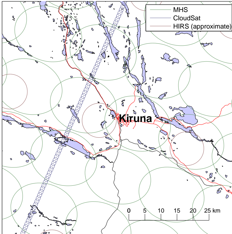
Illustration of sensor footprints over the Kiruna region
