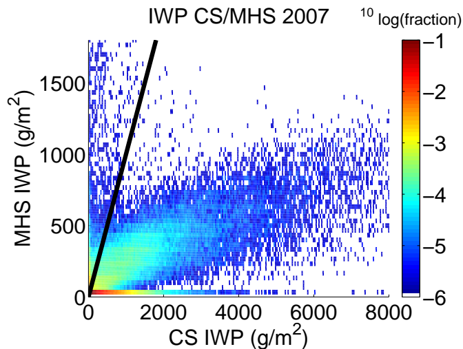
Fig. 6. Two-dimensional histogram of CloudSat Ice Water Path (averaged over an AMSU pixel) and NOAA NESDIS MSPPS IWP, for all collocations in the year 2007. The figure is similar to a scatter plot, but it shows the density of points rather than the actual points. Only measurements where either value is nonzero are shown. The black line shows the ideal case. The colour axis is logarithmic. See text for a discussion.
