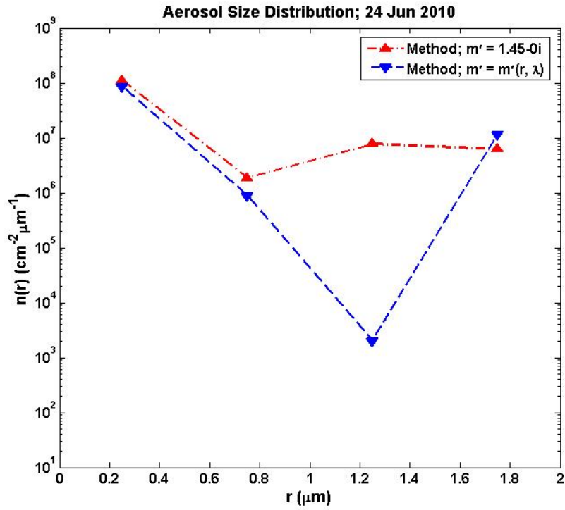
Fig. 3. Daily-averaged aerosol size distribution (1/cm 2 micron) for 24 June 2010 for Zanjan, Iran. Our method is employed with old and new refractive indices respectively.
