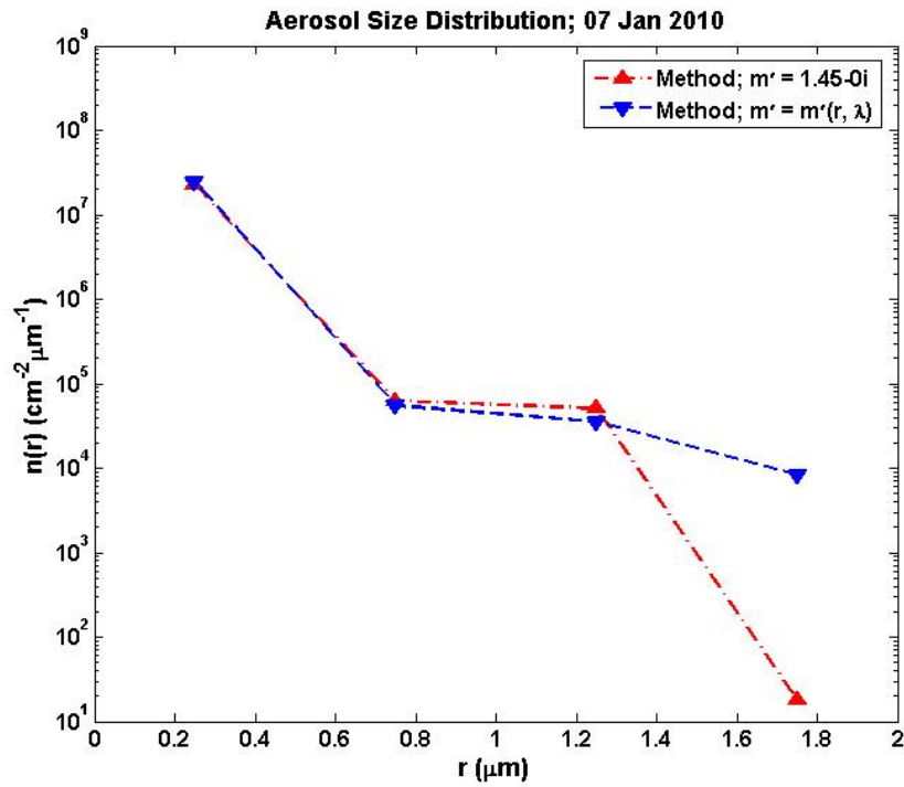
Fig. 1. Daily-averaged aerosol size distribution (1/cm 2 micron) for 7 January 2010 for Zanjan, Iran. Our method is employed with old and new refractive indices respectively.
