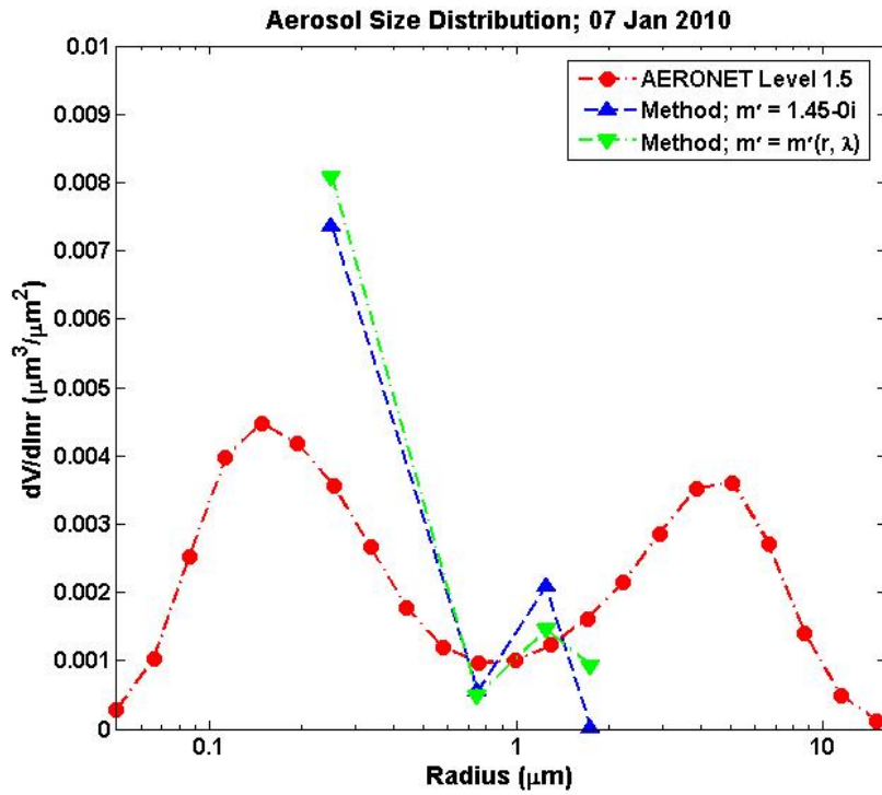
Fig. 2. Daily-averaged aerosol size distribution (micron 3 / micron 2 ) for 7 January 2010 for Zanjan, Iran. AERONET and our method with old and new refractive indices are employed respectively.
