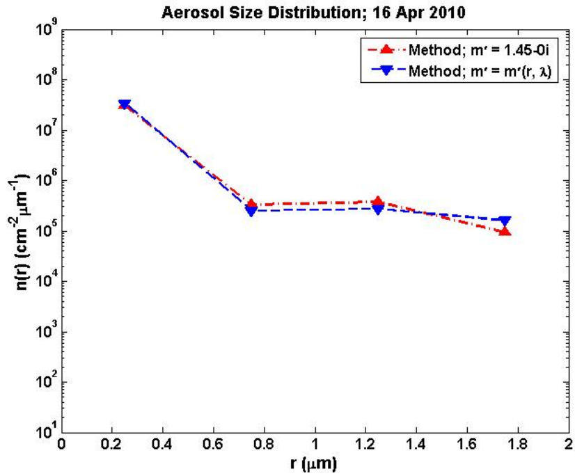
Fig. 5. Daily-averaged aerosol size distribution (1/cm 2 micron) for 16 April 2010 for Zanzan, Iran. Our method is employed with old and new refractive indices respectively.
