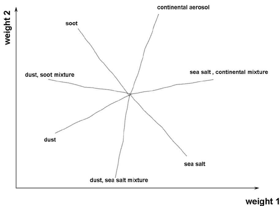
Fig. 1. Uniform distribution of aerosol types in perfect retrieval
