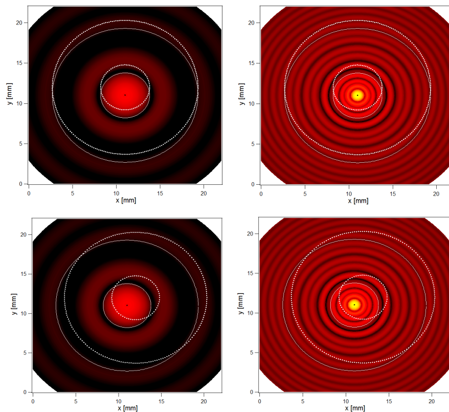
Fig. 4. (S4) Simulated scattered light intensities for 10 \mu\text{m} (left) and 40 \mu\text{m} (right) droplets (see text for full caption)
