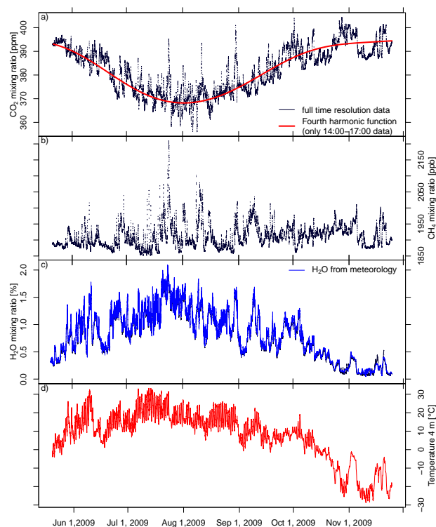
Fig. 1. UPDATE of Fig. 6: ZOTTO time series for (a) CO 2 , (b) CH 4 , and (c) H 2 O for 301m height; (d) temperature.
