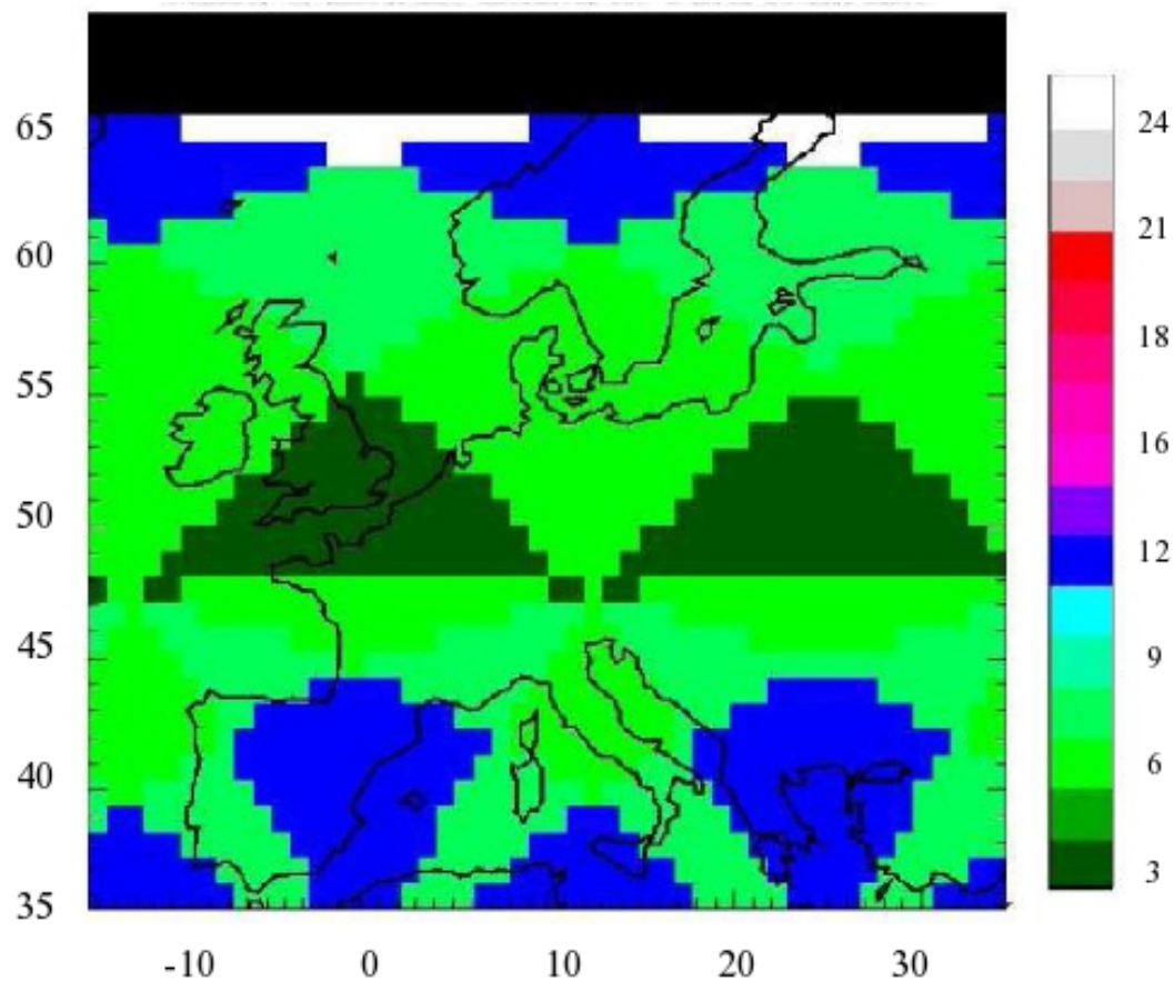
Fig. 1. Useful LEOs optimized (drifted orbits) required for 1 hour revisit time over Europe with a 1^\circ \times 1^\circ resolution ( \sim 100 km)
