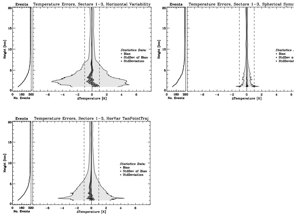
Fig. 1. Dry Temperature error statistics for an ensemble of 306 occultation events, with and without spherical symmetry (from Foelsche et al., 2004b, Fig. 3).
