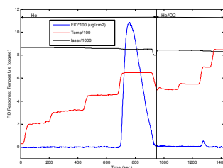
Figure 1: Thermogram obtained from the analysis of \text{CaCO}_3 suspension spiked filter.
