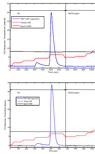
Figure 2: Thermograms obtained from the analysis of two types of natural calcite loaded filters.
