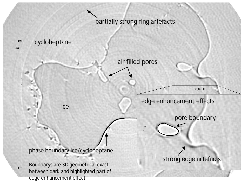
Fig. 1. 1: Unsegmented slice image for the graupel particle #1
