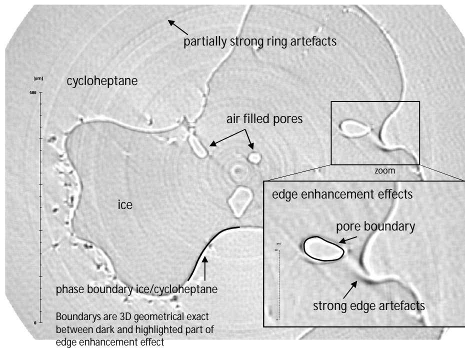
Fig. 1. 1: Unsegmented slice of the ice particle #1
