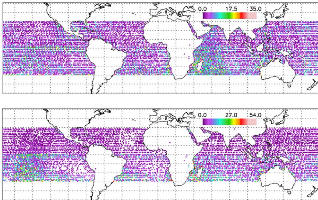
Fig. 1. Day (top) and night (bottom) number of observation counts in 1^\circ latitude and longitude bins.
