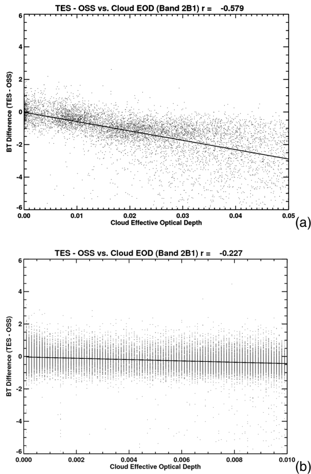
Fig. 2. (a) Relationship between Cloud Effective Optical Depth and Residuals for a Cloud Effective Optical Depth of up to 0.05. (b) Relationship between Cloud Effective Optical Depth and Residuals for a Cloud Effective Optical Depth of up to 0.01.
