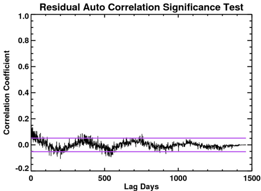
Fig. 5. Significance of auto-correlation in the residuals data – time series is not covariance stationary due to the significance of the auto correlations at ~180, 360 and 540 days.
