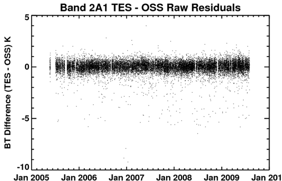
Fig. 3. Brightness temperature differences on a per-spectrum basis. No obvious violation of covariance stationary assumption.
