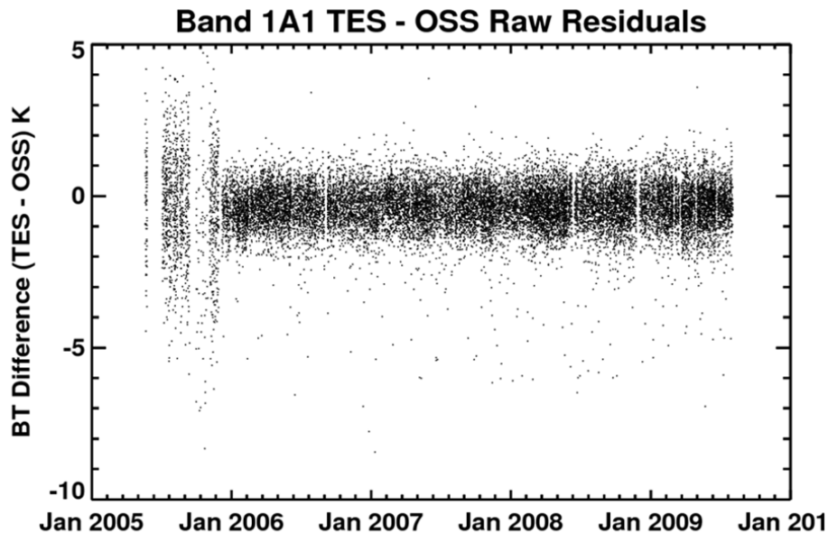
Fig. 7. Optical bench warm-up in late 2005 causes a significant change in the standard deviation of the residuals.
