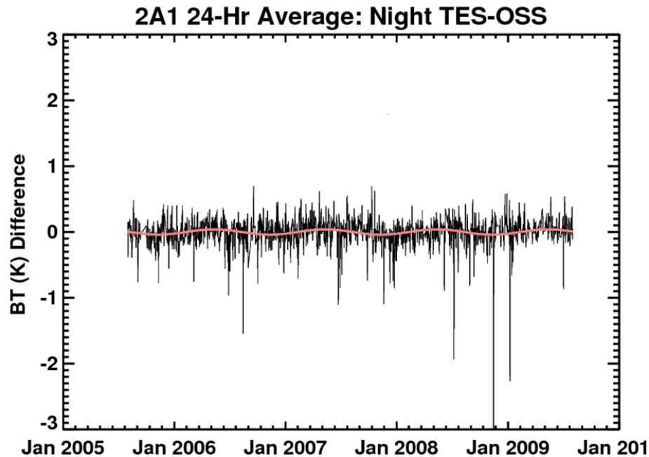
Fig. 6. Daily resolution of a time series containing a yearly harmonic.
