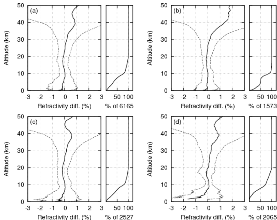
Fig. 3. Statistical comparisons to ECMWF analyses of refractivity derived from GRAS occultations for the first 10 days of December 2010. (a): Global, (b): high latitudes (above 60^\circ ), (c): mid latitudes (between 30^\circ and 60^\circ ), (d): low latitudes (below 30^\circ ). The mean difference (solid) and standard deviation around the mean (dashed) are indicated in the panels to the left, whereas the number of profiles included in the statistics is indicated in the panels to the right.
