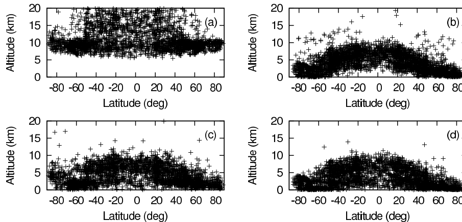
Fig. 4. Penetration depth of GRAS occultations for the first 10 days of December 2010, as a function of latitude. (a) : Rising occultations without “L2 extrapolation”, (b) : setting occultations without “L2 extrapolation”, (c) : rising occultations including “L2 extrapolation”, (d) : setting occultations including “L2 extrapolation”.
