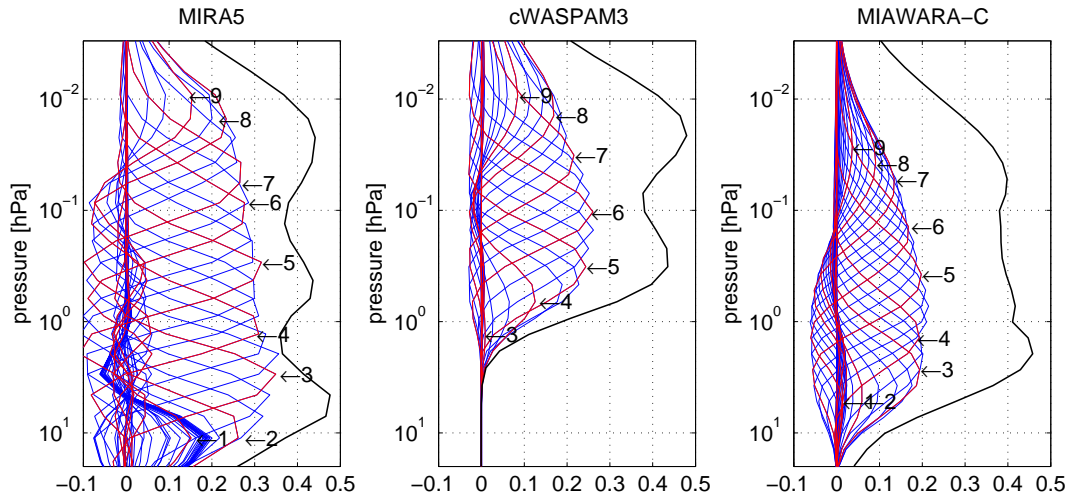
Fig. 5. Averaging kernels and their area (AoA) divided by 2.5 of the single day retrievals on the 2009-02-05. The numbers indicate the AVK belonging to the pressure level closest to 1 = 30 hPa, 2 = 10 hPa, 3 = 3 hPa, 4 = 1 hPa, 5 = 0.3 hPa, 6 = 0.1 hPa, 7 = 0.0 hPa, 8 = 0.01 hPa and 9 = 0.003 hPa.
