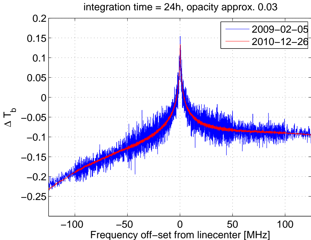
Fig. 11. 1-day integrated spectrum of MIAWARA-C during the ARIS campaign and after the instrumental improvements in the end of 2010. The measurement noise has been improved by a factor of approximately 8 and is hardly visible in the red curve. The difference in the noise level within one spectrum is due to a binning applied to the wings for data reduction. A polynomial of second degree has been removed from the 2010 spectrum to account for the baselines or the different instrumental set-ups.
