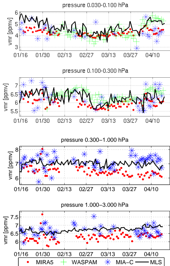
Fig. 9. Time series of middle atmospheric H 2 O for 4 pressure ranges between 3 and 0.03 hPa as observed by MIRA 5, cWASPAM3, MIAWARA-C and MLS. A mean value of the H 2 O-VMR within the pressure ranges indicated is used to account for the different altitude resolution of MLS compared to the ground based instruments.
