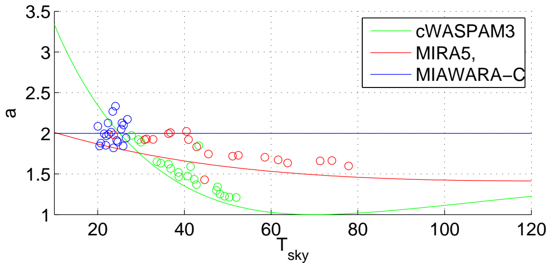
Fig. 2. Sensitivity factor a calculated by Gaussian error propagation on the calibration equations (lines) and from measurements compared to Monte Carlo simulations (circles).
