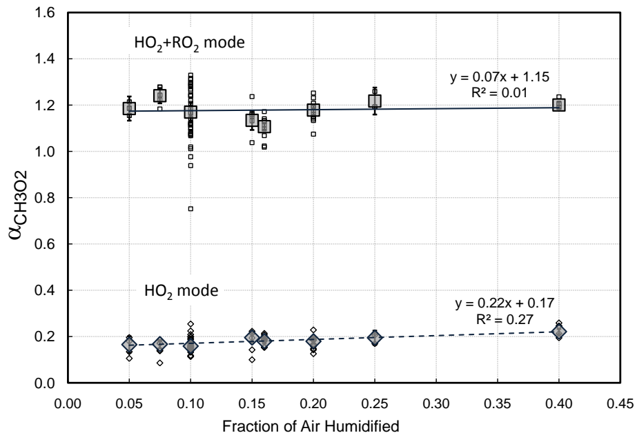
Fig. 4. Dependence of \alpha_{\text{CH}_3\text{O}_2} on the fraction of calibrator air that has been saturated for the HO 2 +RO 2 and HO 2 modes. Smaller points show individual \alpha_{\text{CH}_3\text{O}_2} measurements, and larger points are the error-weighted means of the \alpha_{\text{CH}_3\text{O}_2} determinations at each humidity. Error bars show the error-weighted standard errors.
