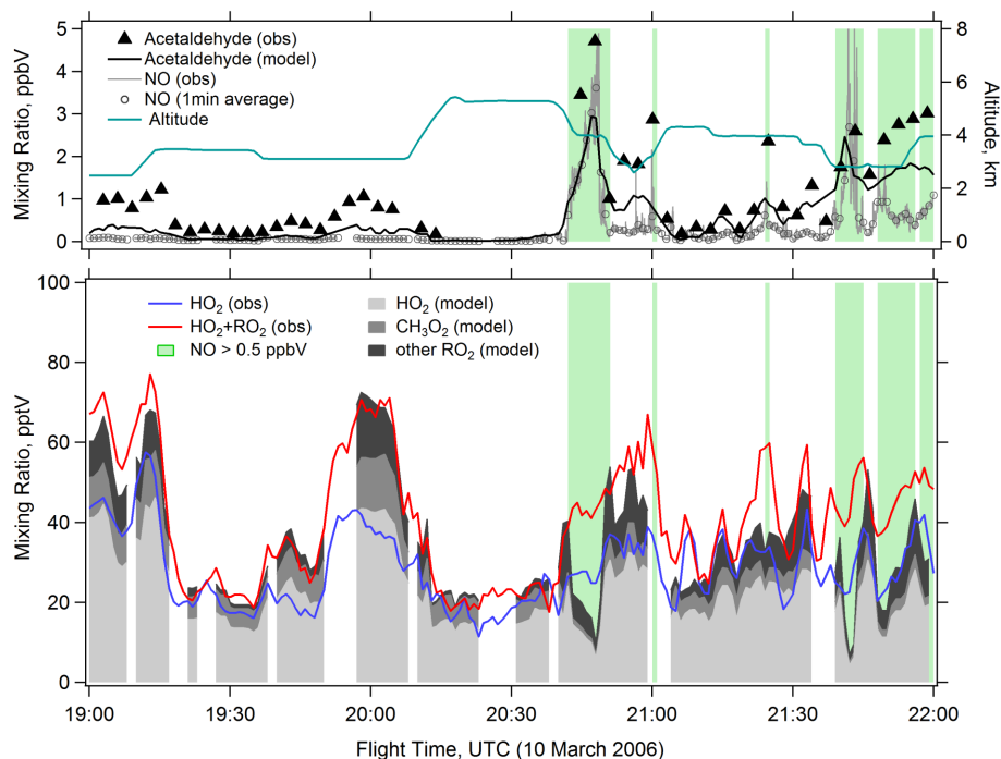
Fig. 9. Time-series plot of the observed and modeled acetaldehyde (top panel) and peroxy radicals (bottom panel) during a section of the flight on 10 March 2006. Local time in the flight region is UTC-6h. Grey areas defined in the legend on the lower plot are stacked modeled [HO 2 ], [CH 3 O 2 ] and non-CH 3 O 2 [RO 2 ]. The 1-s [NO] and 1-min [NO] are both included on the top panel, along with altitude. Time periods when the 1-min average [NO] is greater than 0.5 ppbV are highlighted in green on both plots.
