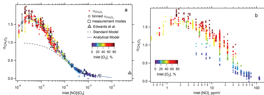
Fig. 3. Plot of measured \alpha_{\text{CH}_3\text{O}_2} against (a) the ratio of [\text{NO}]/[\text{O}_2] in the inlet and (b) inlet [\text{NO}] . Individual measurements are shown as small triangles, colored according to inlet \text{O}_2 concentration. In (a) the open black circles are the average measured \alpha_{\text{CH}_3\text{O}_2} values binned by [\text{NO}]/[\text{O}_2] , with error bars showing the standard deviation for each bin. Squares are the mean \alpha_{\text{CH}_3\text{O}_2} values for the two ambient measurement modes. Large grey triangles are the literature \alpha_{\text{CH}_3\text{O}_2} values reported by Edwards et al. (2003). Also shown are the standard model (dashed curve) and the analytical model (solid blue curve) fit to the results.
