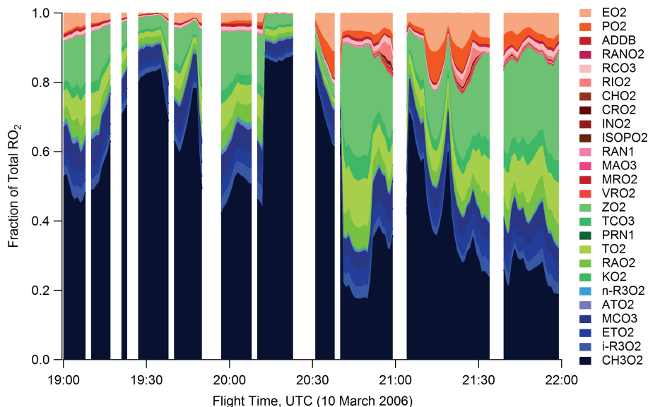
Fig. 10. Time-series plot of modeled RO 2 groups as a fraction of the total RO 2 for the flight on 10 March 2006. Blue-toned groups are those that are primarily measured in the HO 2 +RO 2 mode and not in the HO 2 mode, red-toned groups are those that are likely measured in the HO 2 mode, and green-toned groups are those that contain a mixture of RO 2 that generate signals in the HO 2 and the HO 2 +RO 2 modes. A full description of the RO 2 groups is in Table 6.
