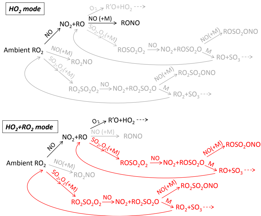
Scheme 1. PerCIMS inlet RO 2 chemistry in the HO 2 mode and HO 2 +RO 2 mode. Reactions in black are known reactions (see text). Reactions in grey are deemed either unimportant or suppressed by competing reactions in a given mode. Reactions in red show proposed chemistry based on inlet chemistry modeling (Sect. 3.2.3).
