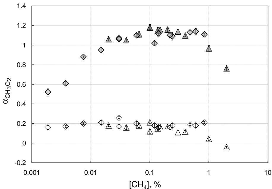
Fig. 7. Dependence of \alpha_{\text{CH}_3\text{O}_2} on CH 4 mixing ratio in the calibration cell. Closed and open symbols are the measured \alpha_{\text{CH}_3\text{O}_2} values at the HO 2 +RO 2 mode and HO 2 mode, respectively, and triangles and diamonds are the results from the single-dilution and double-dilution measurements, respectively. Error bars show the standard errors of each \alpha_{\text{CH}_3\text{O}_2} determination.
