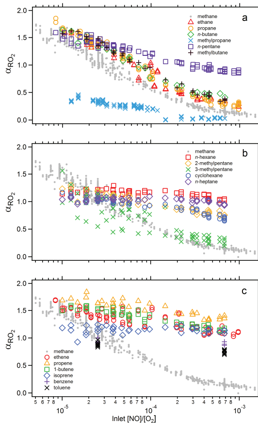
Fig. 8. Plots of \alpha_{RO_2} for RO 2 formed from (a) C 2 –C 5 (i.e., having between two and five carbon atoms) alkane precursors (b) C 6 –C 7 alkane precursors and (c) unsaturated hydrocarbon precursors against the ratio of [NO]/[O 2 ] in the inlet. For comparison, measured \alpha_{CH_3O_2} values are included on each plot.
