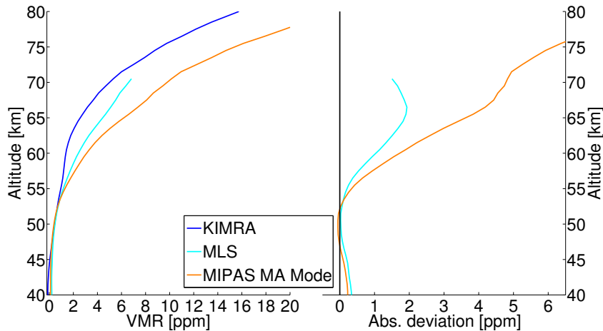
Fig. 15. Comparison of KIMRA with MIPAS (MA mode) and MLS using the collocation criteria R = 1000 km and \Delta PV = 20\% . 9 days with coincidences were found. Left: mean profiles derived according to Sect. 5.1. Right: deviation between the KIMRA and the satellite profiles calculated with Eq. (20).
