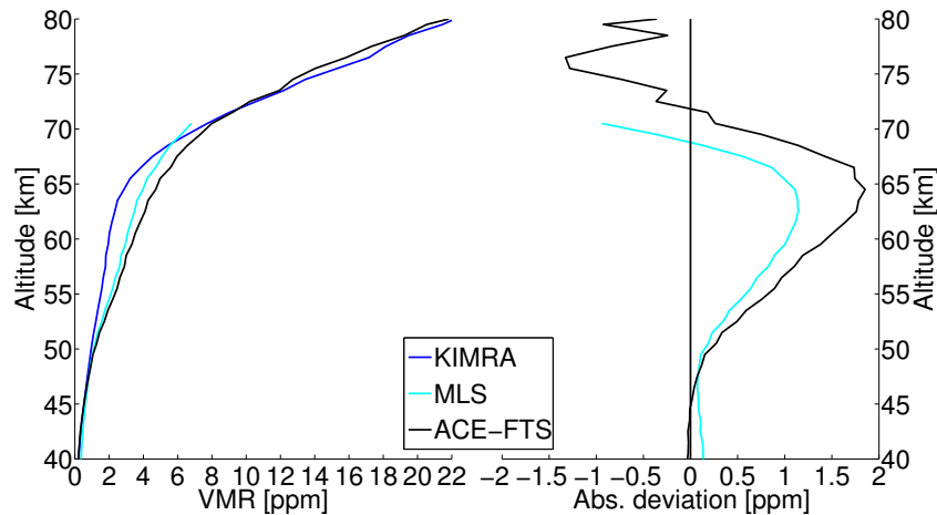
Fig. 14. Comparison of KIMRA with ACE-FTS and MLS using the collocation criteria R = 1000 km and \Delta PV = 20\% . 22 days with coincidences were found. Left: mean profiles derived according to Sect. 5.1. Right: deviation between the KIMRA and the satellite profiles calculated with Eq. (20).
