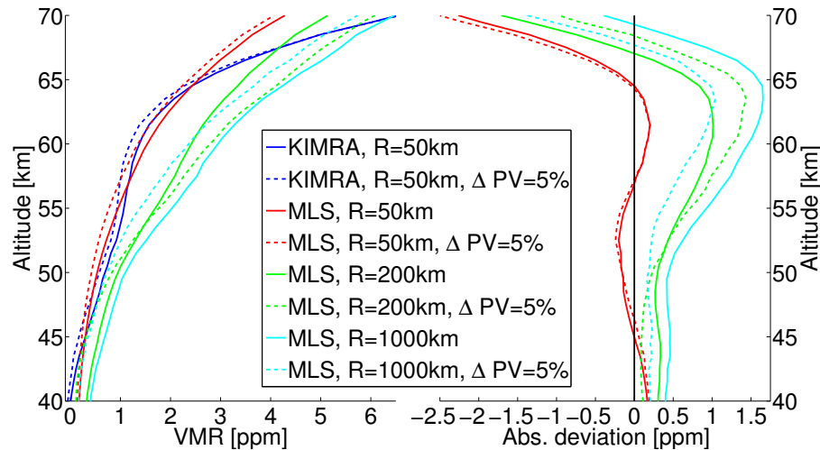
Fig. 10. Investigation of the influence of the collocation area using the MLS dataset. In the first case (solid lines) only the area criterion with different radii R was applied. In the second case (dashed lines) a PV threshold of \Delta PV = 5\% was additionally applied. Left: mean profiles derived according to Sect. 5.1. KIMRA profiles are only shown for the tightest collocation criteria since their sensitivity to a criterion change is low (a dependency only exists, if the averaged period changes as result of a criterion change). Right: deviation between the KIMRA and the satellite profiles calculated with Eq. (20).
