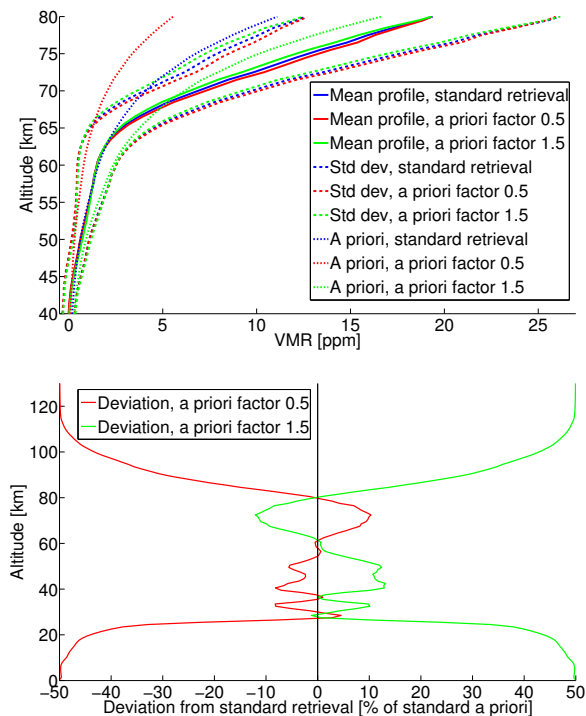
Fig. 8. Test of the retrieval stability when the a priori is changed by a factor of 0.5 or 1.5 respectively. Top: mean profiles, associated standard deviations, as well as a priori profiles for the standard retrieval and the modified retrieval setups in the range of sensitivity between 40 and 80 km. It is obvious, that the change of the mean profile introduced by an a priori change is much smaller than the standard deviation, which is mainly produced by the annual variability. Bottom: deviation of the mean profiles of the modified cases from the standard retrieval profile, plotted for the complete vertical range, normalized with the standard a priori. The deviation is small in the range of sensitivity between 40 and 80 km and approaches, as expected, 50 % where the sensitivity vanishes completely.
