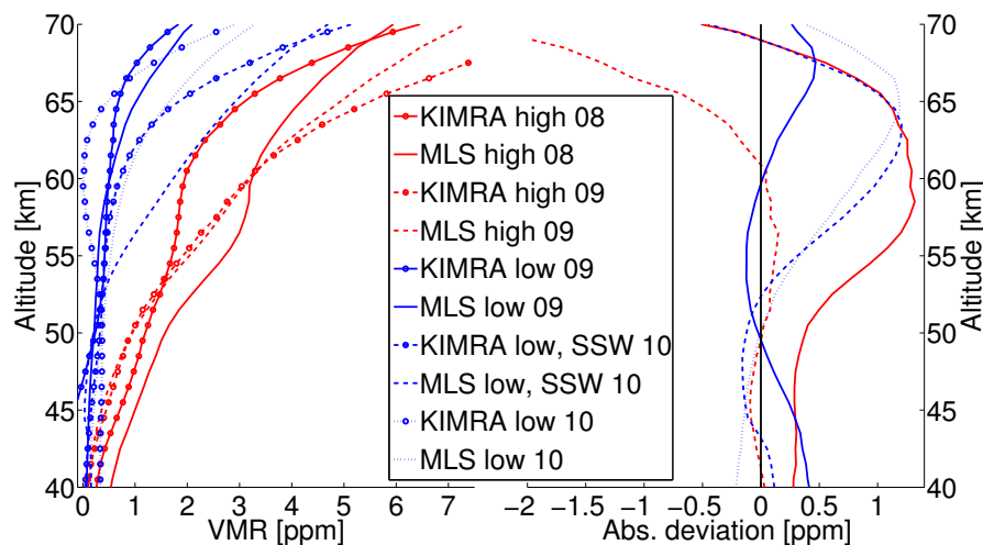
Fig. 12. Investigation of the influence of the averaged period using the MLS dataset. Periods with comparatively high (red) or low (blue) CO values were chosen, for details see Table 5. Left: mean profiles derived according to Sect. 5.1. Right: deviation between the KIMRA and the satellite profiles calculated with Eq. (20).
