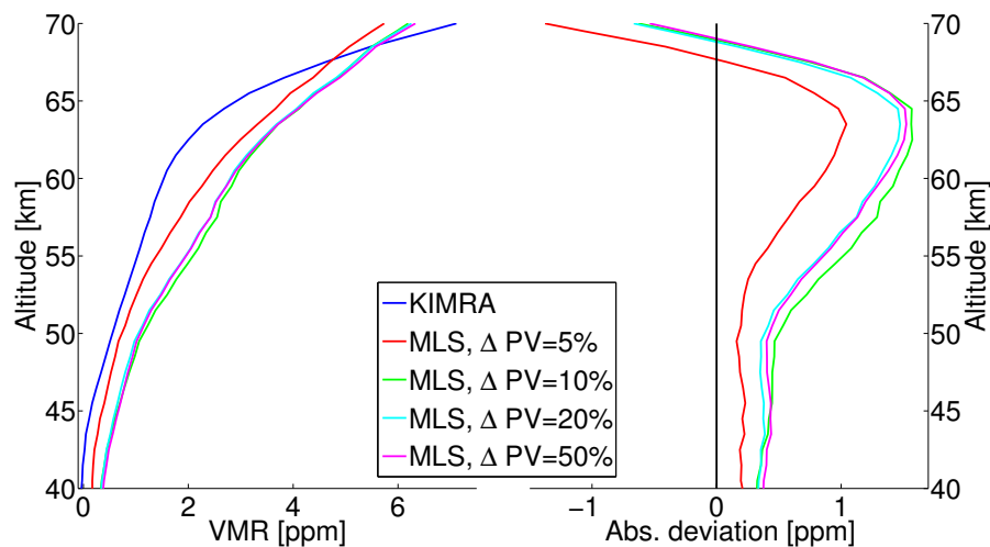
Fig. 11. Investigation of the influence of the PV collocation criterion using the MLS dataset. Left: mean profiles derived according to Sect. 5.1. Right: deviation between the KIMRA and the satellite profiles calculated with Eq. (20).
