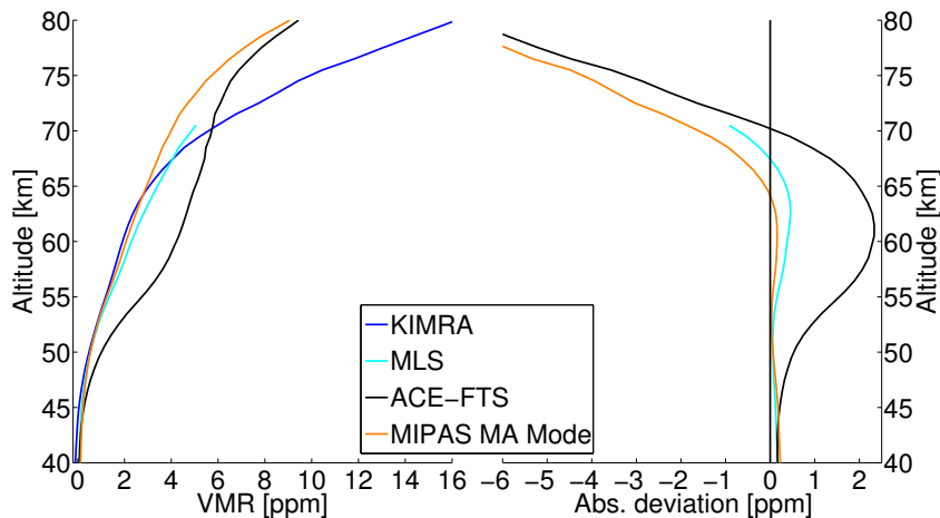
Fig. 16. Comparison of KIMRA with ACE-FTS, MIPAS (MA mode), and MLS using the collocation criteria R = 1000 km and \Delta PV = 50\% . 1 day with coincidences was found. Left: mean profiles derived according to Sect. 5.1. Right: deviation between the KIMRA and the satellite profiles calculated with Eq. (20).
