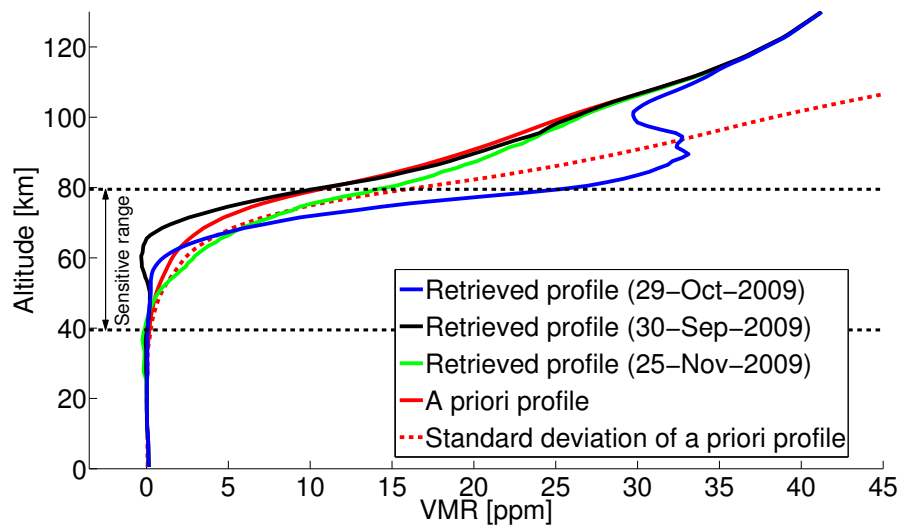
Fig. 3. Retrieved CO profiles (selected to cover the complete range of the CO change during a winter), as well as the constant a priori profile and its standard deviation represented by \sqrt{S_a^{ii}} . The range of sensitivity of the KIMRA CO measurements (Sect. 3.4) is marked with black dashed lines. Out of this range the profiles are not reliable, but are shown here for a complete demonstration of the retrieval results.
