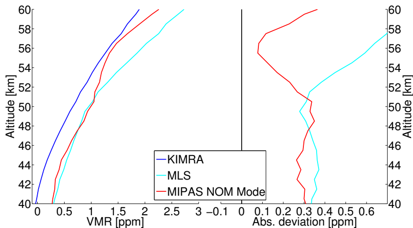
Fig. 13. Comparison of KIMRA with MIPAS (NOM mode) and MLS using the collocation criteria R = 250 km and \Delta PV = 20\% . 42 days with coincidences were found. Left: mean profiles derived according to Sect. 5.1. Right: deviation between the KIMRA and the satellite profiles calculated with Eq. (20).
