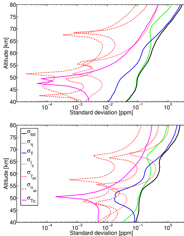
Fig. 7. Typical examples of error contributions. The dominating contributions to the total error \sigma_{\text{tot}} come from the measurement noise error \sigma_{\eta} , from the temperature error \sigma_T , and frequently from the spectroscopic error \sigma_{l_0} . Top: example of 29 October 2009, which has no dominating spectroscopic contribution. Bottom: example of 4 February 2009, which shows a pronounced spectroscopic contribution at approx. 60 km.
