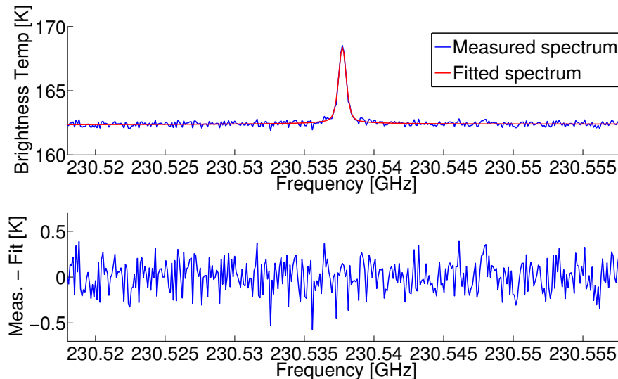
Fig. 2. Top: spectrum measured on 29 October 2009, 06:52 h, together with the fit calculated by the retrieval process. Bottom: the corresponding residuum (difference of the measured spectrum and the fitted spectrum), which contains only noise contributions, showing that the CO line was fitted adequately.
