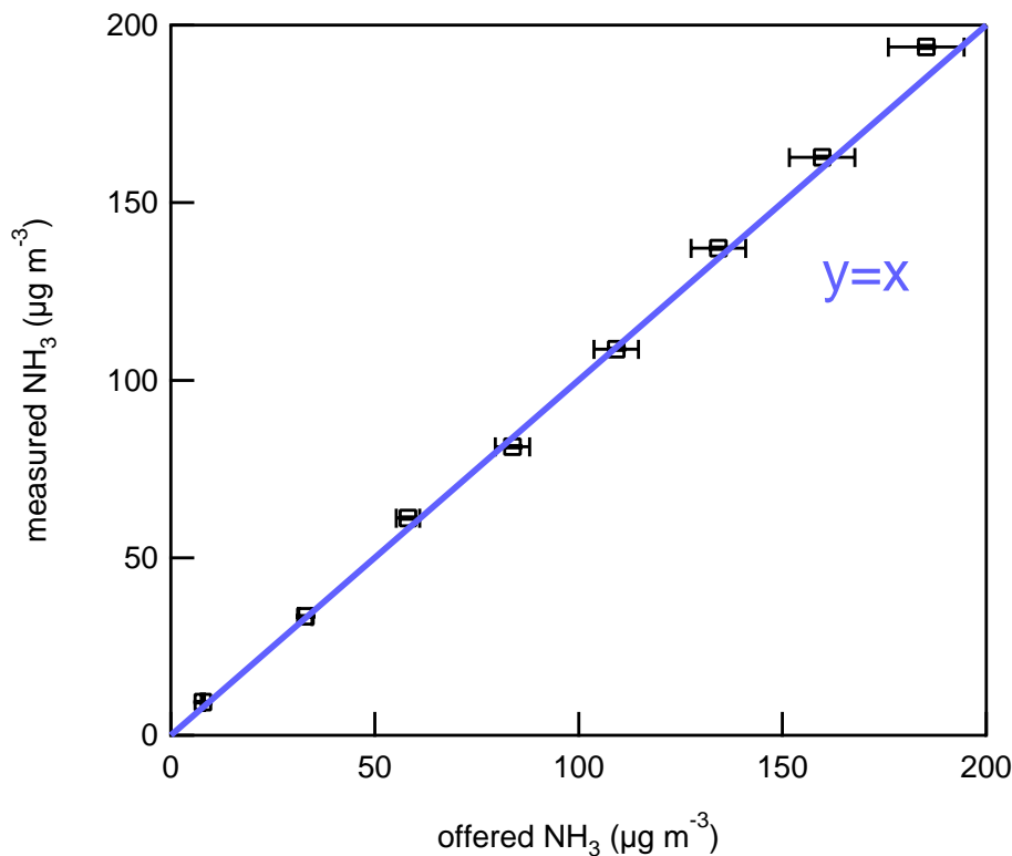
Fig. 9. Results of the linearity test for the RIVM DOAS instrument. Horizontal error bars indicate estimated errors of 5% in the NH 3 concentrations offered. Vertical error bars indicate 1- \sigma errors in the measured NH 3 concentrations. If the error bars are not visible they are smaller than the symbol plotted.
