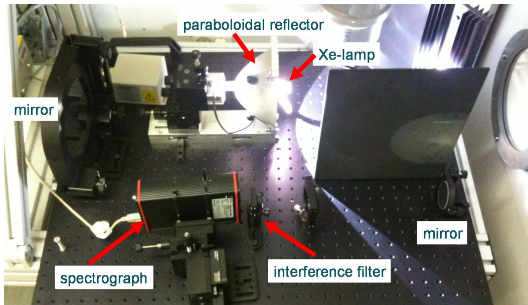
Fig. 7. Photograph of the miniDOAS breadboard instrument.
