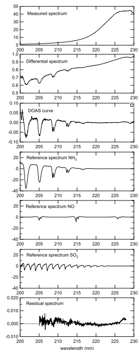
Fig. 8. Measurement analysis shown for a typical measurement. From top to bottom: measured spectrum (5-min average), differential spectrum ( I_{o,\lambda}/I_{\lambda} ), DOAS curve ( \ln[\frac{I_{o,\lambda}/I_{\lambda}}{(I_{o,\lambda}/I_{\lambda})_{\text{boxcar}}}] ), \text{NH}_3 , \text{NO} , and \text{SO}_2 reference spectra used in the fitting procedure, and the residual spectrum. Scales for the y-axes are arbitrary. Units for the reference spectra of \text{NH}_3 , \text{NO} , and \text{SO}_2 are the same. For these measured reference spectra the concentrations were equivalent to ambient concentrations over a path length of 100 m of 200 \mu\text{g m}^{-3} for \text{NH}_3 , 570 \mu\text{g m}^{-3} for \text{NO} , and 50.6 \mu\text{g m}^{-3} for \text{SO}_2 . The residual spectrum is plotted in the same units as the DOAS curve. It is a tool that helps to identify potential flaws in the measurements, such as interference problems.
