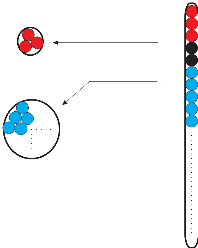
Fig. 4. The optical fiber bundle is a spot/spot to slit line bundle assembly. The end going to the spectrograph consists of 47 fibers formatted into a slit line. The other end of the bundle is divided into two legs. One leg contains the top 3 fibers from the slit line formatted into a spot. This end leads to the zinc lamp. The next 2 fibers from the slit line are intentionally dark (dead). The other leg consists of the remaining 42 fibers formatted into a spot. The light of the telescope is focussed on this spot.
