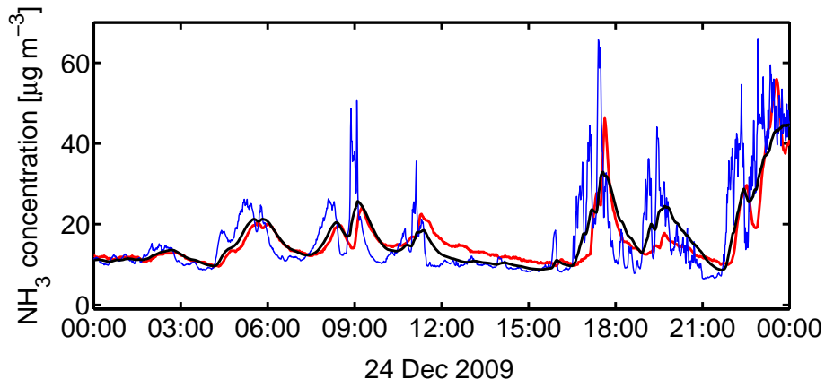
Fig. 21. Minute values of the miniDOAS (blue curve), and the AMOR (red curve) compared to delayed and smoothed miniDOAS data (black curve). Both the miniDOAS data and the delayed and smoothed miniDOAS data have been augmented with an offset of 3.4 \mu\text{g m}^{-3} .
