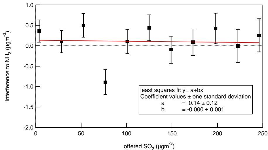
Fig. 11. Results of the \text{SO}_2 interference test for the RIVM DOAS instrument.
