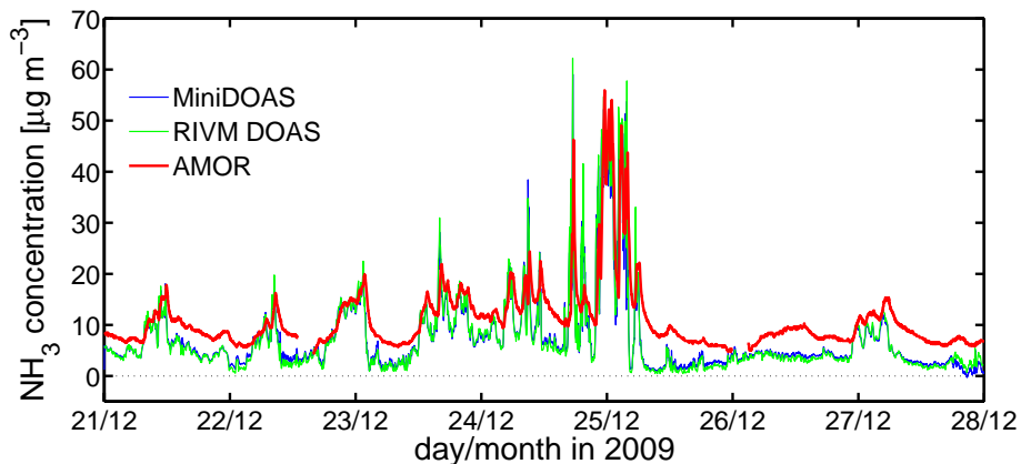
Fig. 17. RIVM DOAS (green line; 5-min values), miniDOAS (blue line; 1-min values), and AMOR data (red line; 1-min values) obtained in the field in Vredepeel from 21 to 28 December 2009.
