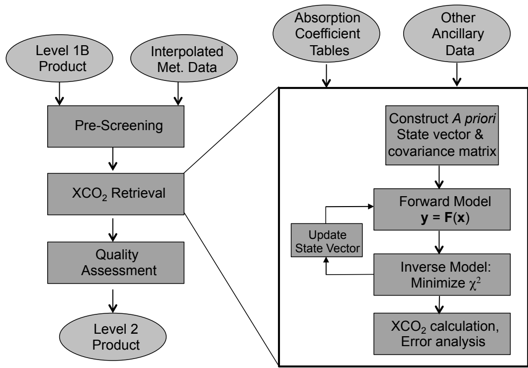
Fig. 1. Flowchart showing the basic steps for the end-to-end ACOS Level-2 algorithm.
