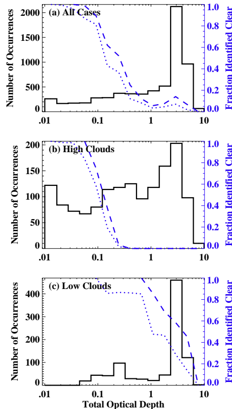
Fig. 6. Panel (a): distribution of cloud plus aerosol optical depth (AOD) for the synthetic orbits (solid line) and fraction of scenes identified as clear by the cloud screening algorithm (dashed and dotted lines). The dashed line shows the result for the operational thresholds, while the dotted line shows the result when the |\Delta P_{\text{cid}}| threshold is tightened to 10 hPa. Panel (b): Same as panel (a), but only shows those cases where 95 % of the AOD resides in the upper 40 % of the atmosphere (high clouds). Panel (c): Same as panel (a), but only shows those cases where 95 % of the AOD resides in the lowest 30 % of the atmosphere (low clouds).
