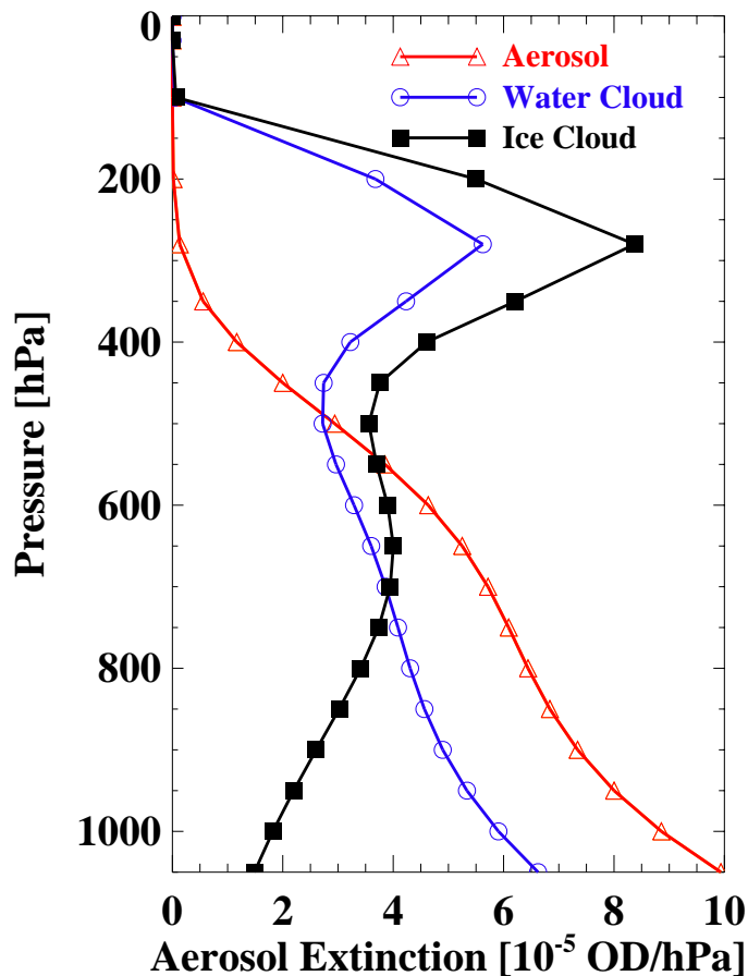
Fig. 3. A priori extinction profiles of cloud and aerosol at 0.755 \mu m wavelength. The two formal aerosol types each have the same a priori profile and are shown here as “Aerosol”. The algorithm formally retrieves the logarithm of this quantity.
