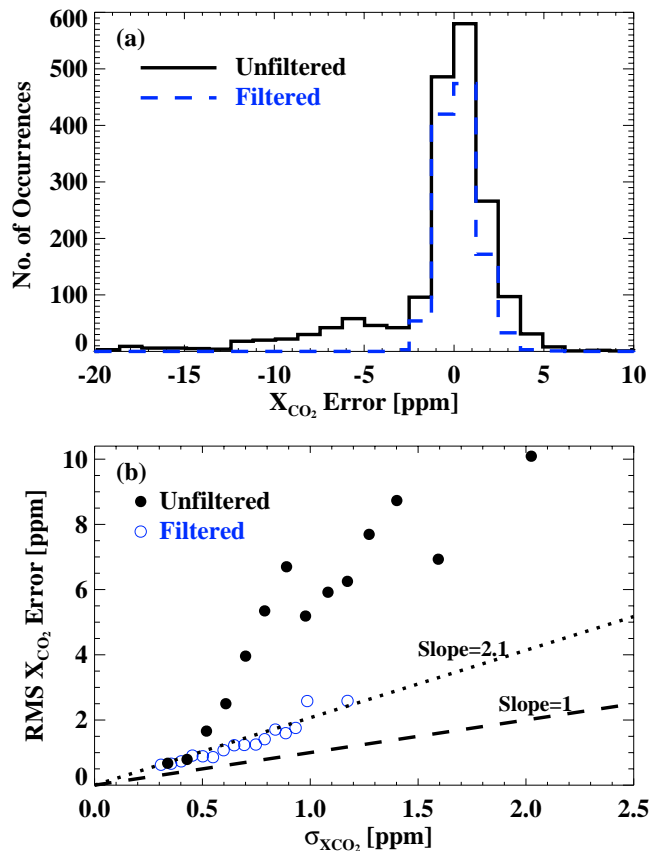
Fig. 12. (a) Histogram of test 6 X_{CO_2} errors, for both unfiltered retrievals (black, solid) and those passing the post-processing filters (blue, dashed). (b) Plot of test 6 actual RMS errors in X_{CO_2} vs. a posteriori error \sigma_{X_{CO_2}} , calculated by binning X_{CO_2} error in bins of \sigma_{X_{CO_2}} . The one-to-one line (dashed) would be expected if the a posteriori error fully explained the true errors; the best-fit line for the filtered retrievals (dotted) has a slope of 2.1.
