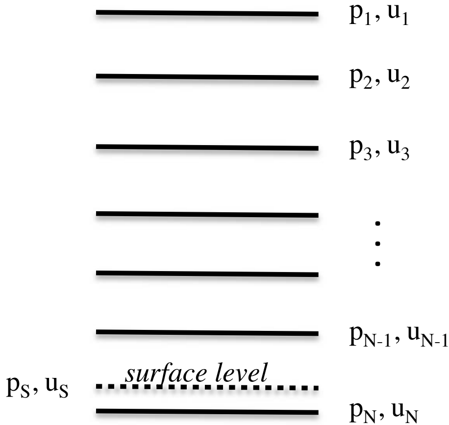
Fig. A1. The standard, pre-defined pressure levels are given by p_i, i = 1 \dots N . At each level i there is a corresponding value of retrieved \text{CO}_2 volume mixing ratio given by u_i . The dotted line represents the surface level.
