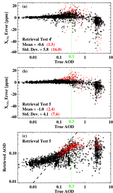
Fig. 8. (a) Retrieved X_{\text{CO}_2} error versus true AOD for test 4. Black circles denote converged retrievals which passed the cloud filter; red dots denote converged retrievals which failed the cloud filter. The corresponding mean and RMS X_{\text{CO}_2} errors in ppm are given in the lower left. The green, vertical dashed line denotes the original 0.3 AOD threshold for retrievals identified in Crisp et al. (2004). (b) Same as panel (a), but for test 5. (c) The retrieved AOD versus true AOD in test 5. The one-to-one line (dashed) is shown for reference.
