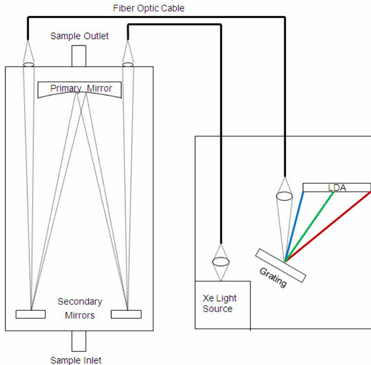
Fig. 1. A schematic of the benchtop AE-DOAS system. Light from the xenon lamp in the rack mountable spectrometer (shown on the right) is focused onto a fiber optic cable for transfer into the multi-pass gas cell (shown on the left). After a number of passes in the gas cell, the reflected light is focused onto a second fiber optic cable and detected by the spectrometer. The spectrometer consists of a grating and a 3078 element linear diode array. The typical gas cell path length is 19.51 m, unless otherwise noted.
