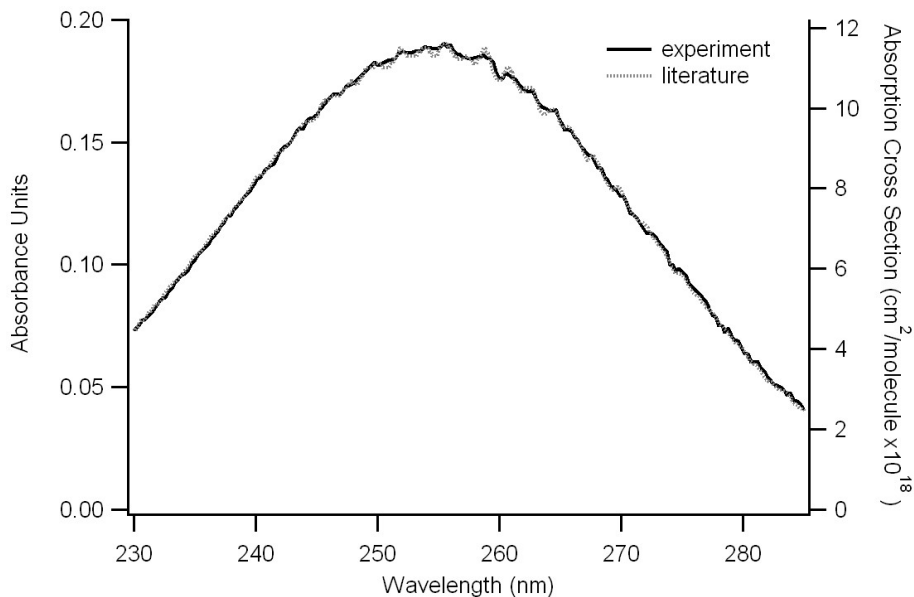
Fig. 4. The UV absorption spectrum of the Hartley band of ozone measured with an AE-DOAS path length of 9.75 m is shown as a solid black line. This is compared to the dotted grey line showing the absorption cross section spectrum of ozone (shown on the right y-axis) (Bogumil et al., 2003). A wavelength adjustment equivalent to adding one nanometer to the experimental spectrum is required to match the fine spectral structure seen in the literature spectrum.
