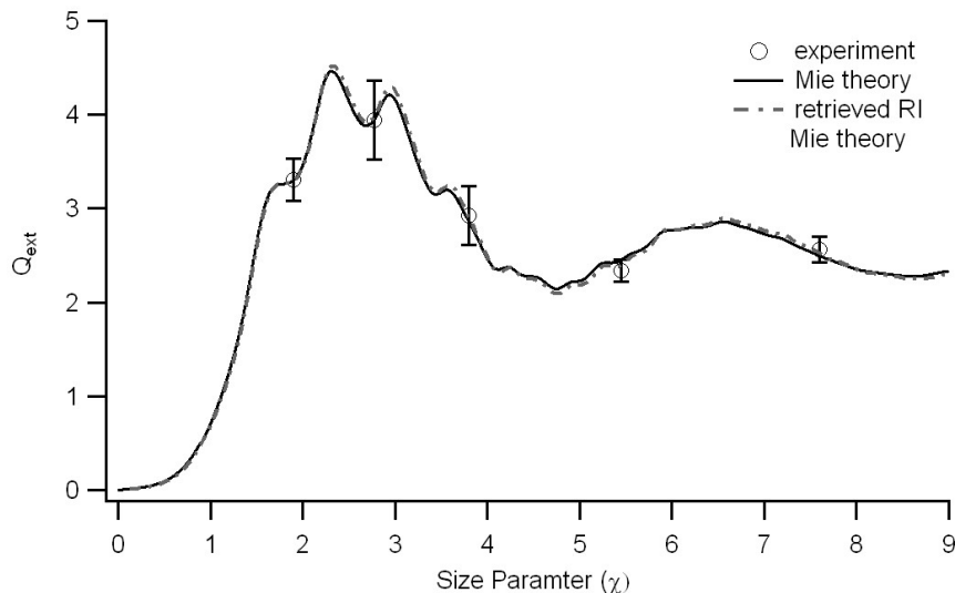
Fig. 7. The experimentally measured Q_{\text{ext}} versus size parameter for PSL at a wavelength of 248 nm are shown as open circles. The black line is the Mie theory calculation performed with a CRI from French et al. (2007) ( m = 1.826 + 0.059i at \lambda = 248 nm). The grey dot-dash line is the Mie theory calculation for the CRI retrieved from the experimental data ( m = 1.82 + 0.05i ). The experimental extinction efficiency is reported for PSL diameters of 150 nm, 220 nm, 300 nm, 430 nm, and 600 nm (from left to right) and the reported error bars are 1\sigma for repeat measurements.
