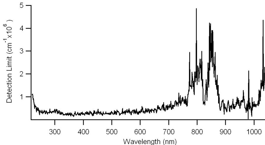
Fig. 2. The AE-DOAS detection limit is shown as a function of wavelength. This data is smoothed by averaging over five recorded wavelength values. It is clear that the detection limit is steady over the center of the solar spectrum from 235–700 nm. At wavelengths outside this range, the detection limit increases due to low lamp intensity.
