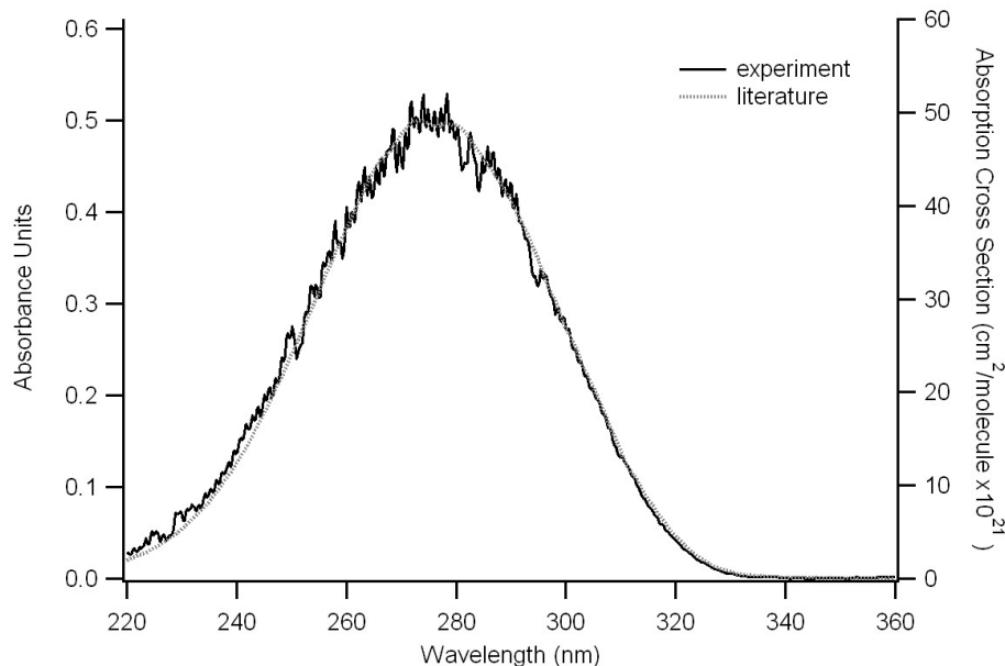
Fig. 5. The UV absorption spectrum obtained with the AE-DOAS of acetone with a 5-point boxcar average is shown as a solid black line. This is compared with the dotted grey line showing the absorption cross section spectrum of gas phase acetone (shown on the right y-axis) (Meyrahn et al., 1986).
