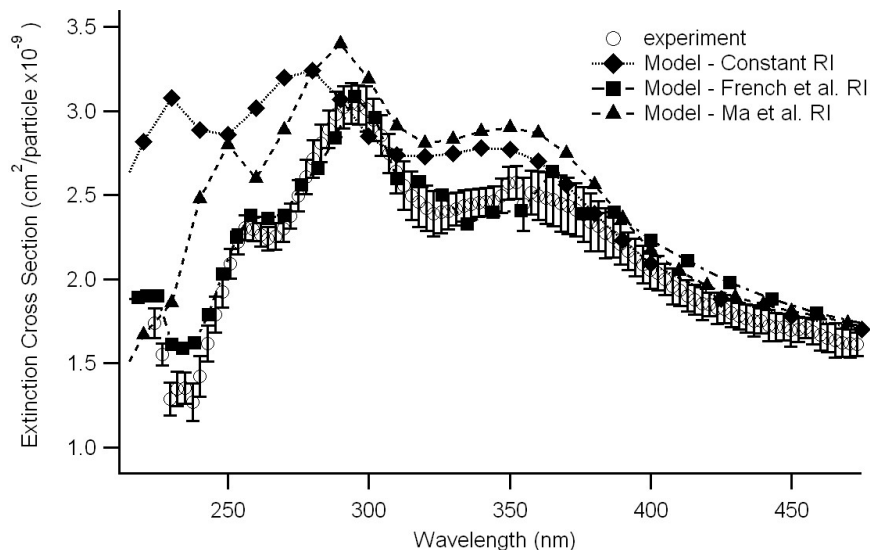
Fig. 6. The extinction cross section spectrum measured by the AE-DOAS for 300 nm PSL is shown as open circles. The experimental error bars represent 1\sigma of the mean. Mie theory calculations are performed with various values for the RI. The result based on the constant manufacturer's reported RI is shown as solid diamonds, the RI derived from Ma et al. (2003) based on the Cauchy coefficients is shown as solid diamonds and French et al.'s (2007) experimentally determined CRI is solid squares. The calculations show improved convergence at wavelengths greater than 475 nm and are therefore not shown.
