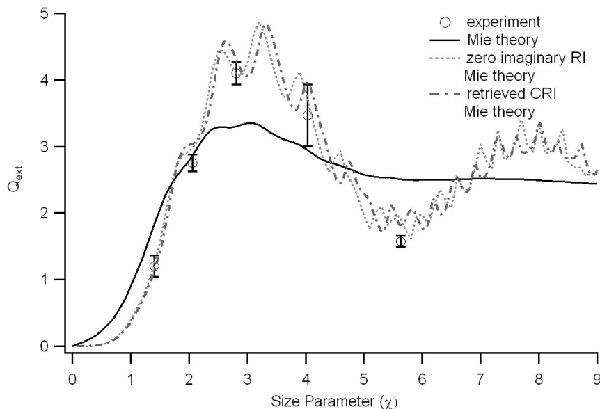
Fig. 8. At a wavelength of 335 nm, the Q_{\text{ext}} measured by the AE-DOAS (open circles) does not match the Q_{\text{ext}} predicted by Mie theory generated with the French et al. (2007) CRI ( m = 1.686 + 0.197i ) shown as the black line. The Mie theory generated when the imaginary portion of this CRI is reduced to zero is shown in the light gray dotted line. The grey dot-dash line is the Mie theory calculation for the CRI retrieved from the experimental data ( m = 1.72 + 0.005i ). Errors bars are 1\sigma on repeat experimental measurements.
