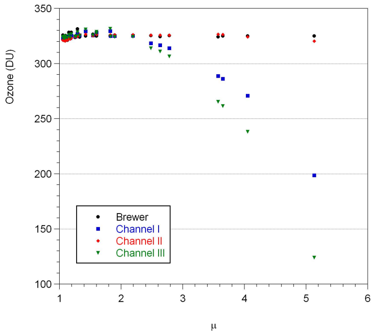
Fig. 4. Instantaneous ozone values from Brewer and the three Microtops II channels on 12 May 2009 in Lampedusa.
