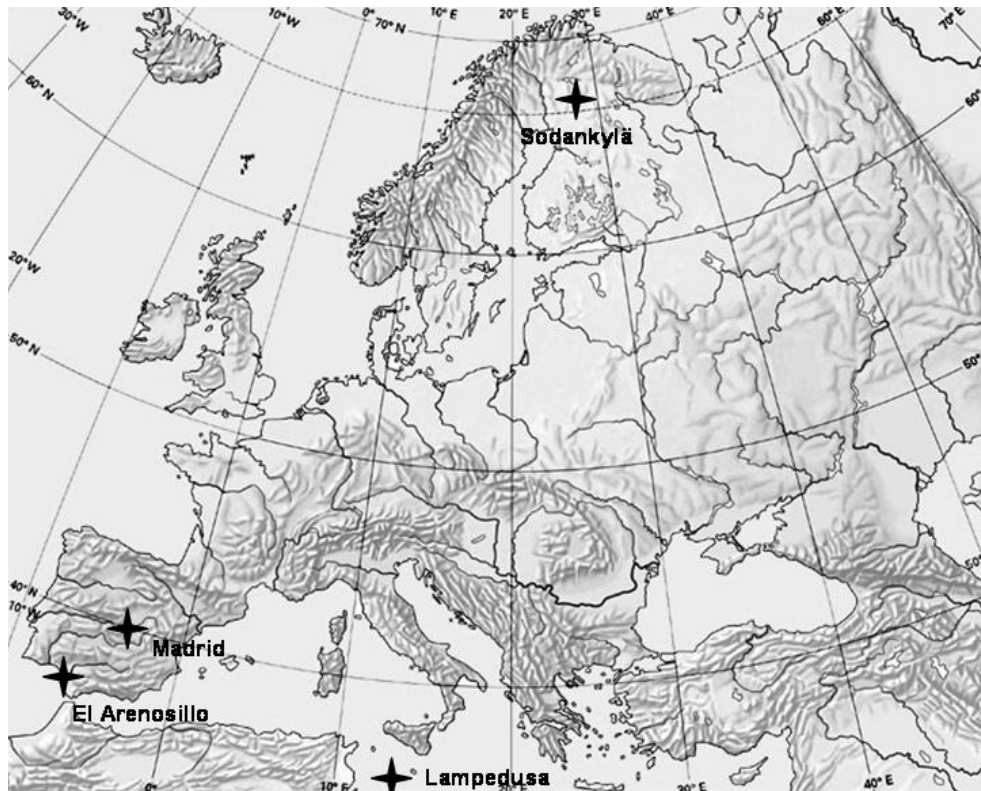
Fig. 1. Geographic map of the measurement sites.
