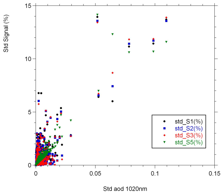
Fig. 3. Scatter plot of the standard deviation of the Microtops II signals at 305, 312, 320 and 1020 nm against the standard deviation of AOD 1020 .
