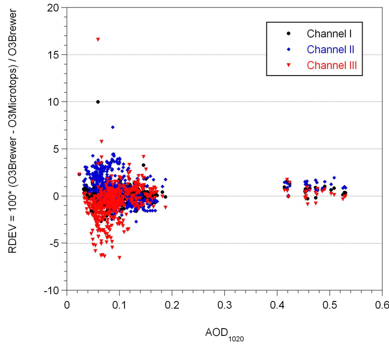
Fig. 7. Instantaneous relative deviation between Brewer and Microtops II ozone against AOD_{1020} . Only data for airmass smaller than 3 are included.
