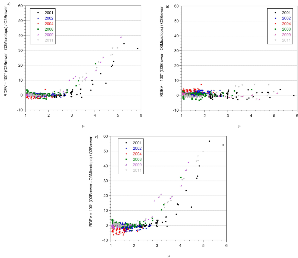
Fig. 6. Airmass evolution of the instantaneous relative deviation between Brewer and Microtops II ozone: (a) Channel I, (b) Channel II, and (c) Channel III.
