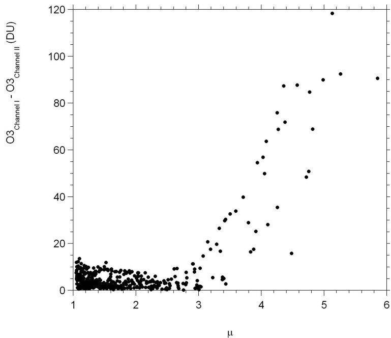
Fig. 5. Difference between Microtops Channel I and Channel II retrievals versus the airmass.
