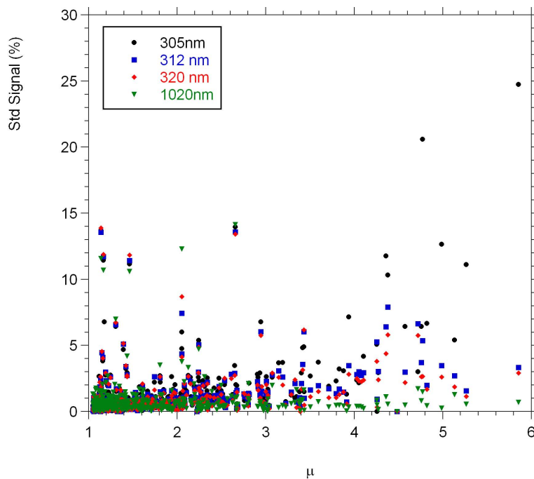
Fig. 2. Standard deviation of the Microtops II signals at 305, 312, 320, and 1020 nm against the airmass. Data from all the field campaigns are shown.
