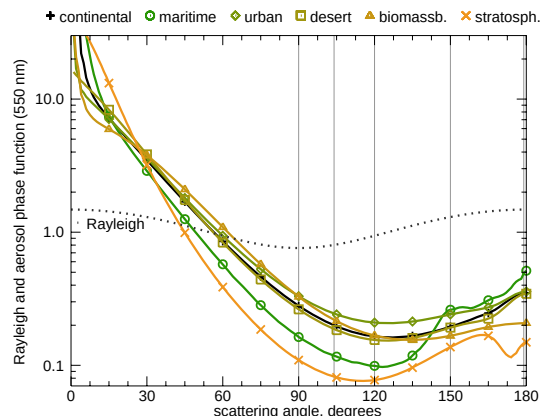
(a) Separated Rayleigh and aerosol phase functions
