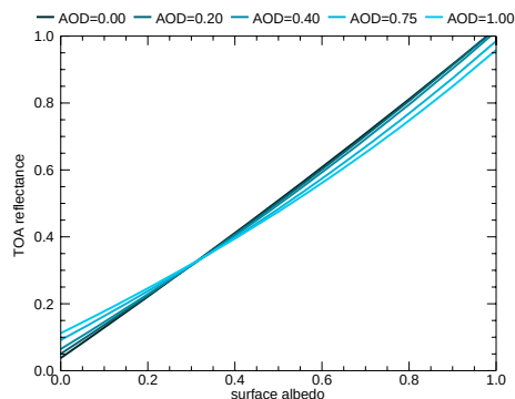
(c) Desert aerosol model at 550 nm
