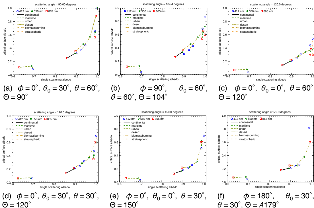
Fig. 6: CSA as function of SSA for AOD = 0.2 at 412 nm, 550 nm and 865 nm, as well as for different aerosol types and different combinations of viewing azimuth angle \phi , solar zenith angle \theta_0 , viewing zenith angle \theta and the corresponding scattering angle \Theta .
