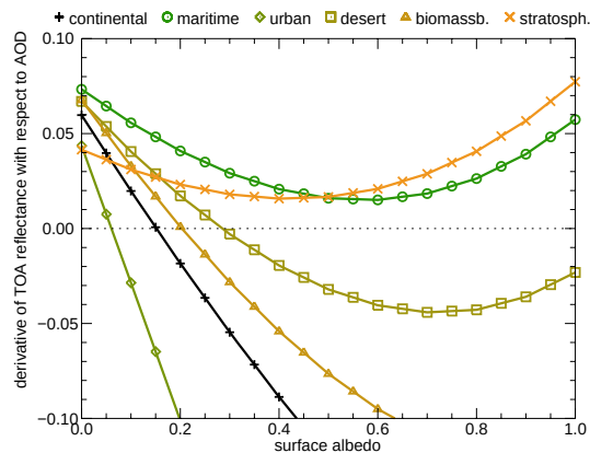
(b) AOD = 0.2
