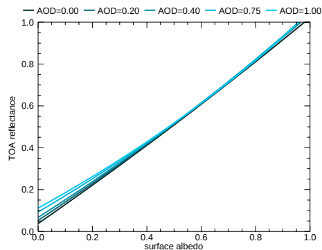
(a) Maritime aerosol model at 550 nm
