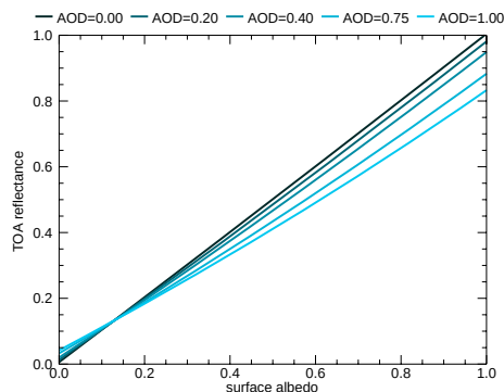
(c) Continental aerosol model at 865 nm
