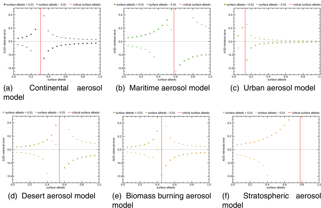
Fig. 8: AOD retrieval error ( \tau_{\text{true}}^{\text{aer}} - \tau_{\text{retrieved}}^{\text{aer}} ) as a function of surface albedo at 550 nm for different aerosol types with \tau_{\text{true}}^{\text{aer}} = 0.3 at \phi = 0^\circ , \theta_0 = 30^\circ , and \theta = 30^\circ . The plus signs denote an overestimation of surface albedo by +0.01 and the minus signs an underestimation of surface albedo by -0.01. The CSA is provided by the red line.
