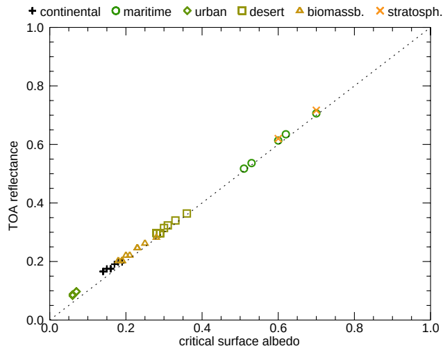
Fig. 5: TOA reflectance R_{550\text{nm}}^{\text{TOA}}(\tau_{550\text{nm}}^{\text{aer}} \in [0.0, 0.05, 0.1 (0.1) 0.5, 0.75, 1.0]) according to Eq. (1) as a function of CSA. Solar zenith angle is 0^\circ , viewing zenith angle 30^\circ and scattering angle 150^\circ .
