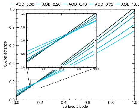
(b) Continental aerosol model at 550 nm
