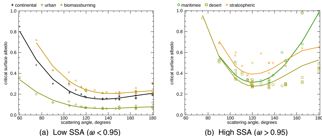
Fig. 7: CSA as a function of scattering angle for AOD = 0.2 at 550 nm. Certain combinations of solar and observing geometries have the same scattering angle, which leads to multiple results per aerosol model, especially for less absorbing aerosol types.
