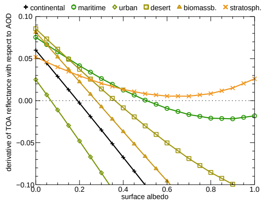
(c) AOD = 1.0
