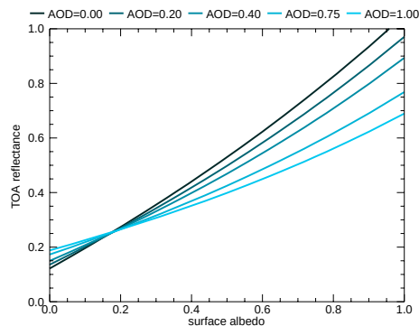
(a) Continental aerosol model at 412 nm
