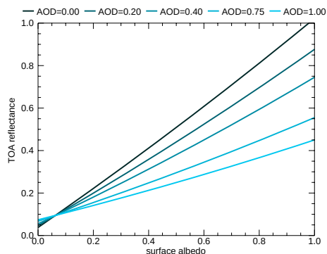
(b) Urban aerosol model at 550 nm
