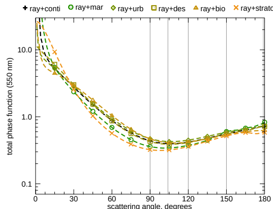
(b) Total phase functions
