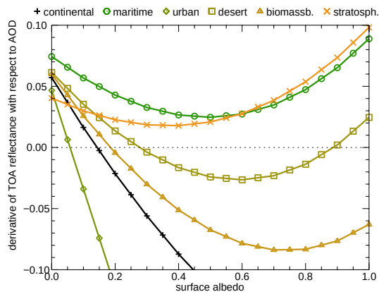
(a) AOD = 0.05
