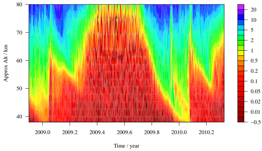
Fig. 1. Time series of MLS CO in a 5 degree latitude by 24 degree longitude region centred on Kiruna.
