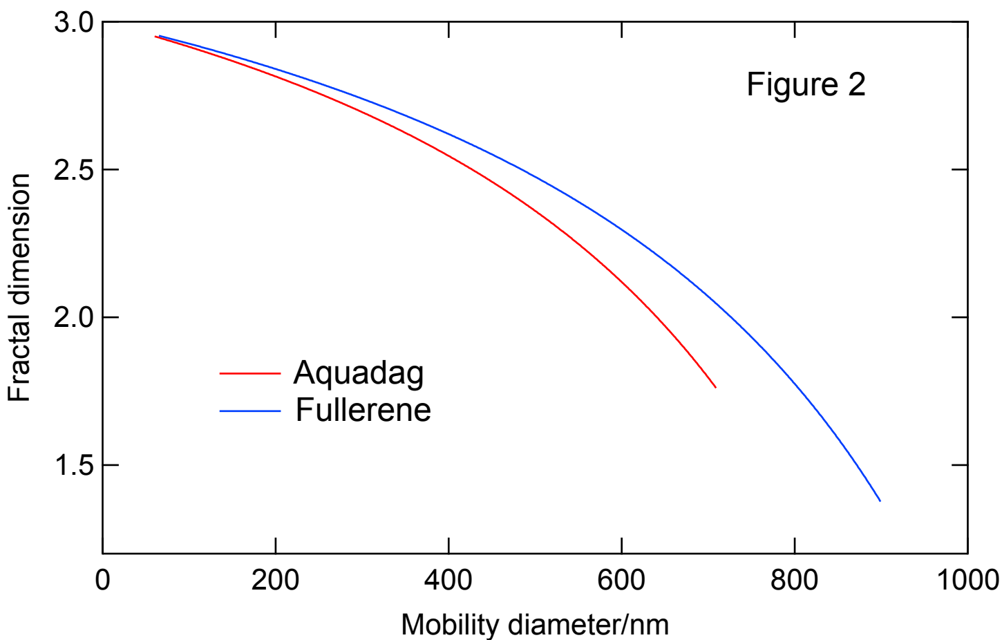
Fractal dimension for particles of Aquadag and Fullerene calculated from the linear fits.
