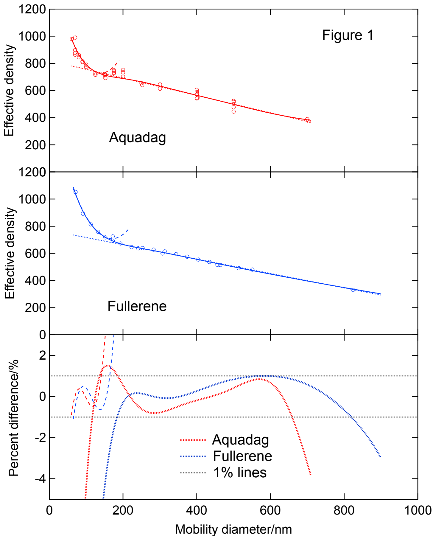
Effective density of Aquadag (top panel) and Fullerene (middle panel) particles as a function of mobility diameter. Solid lines are polynomial fits by Gysel et al., dotted lines are linear fits, and dashed lines are quadratic fits at low values of mobility diameter (the linear and quadratic fits are so close to those of Gysel that they are nearly obscured by the solid lines). Errors of the fits (as percent differences) are shown in lower panel.
