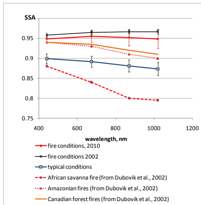
Fig.9. Spectral dependence of aerosol single scattering albedo (SSA) for Moscow fire conditions in 2010, 2002, and typical conditions with error bars at 95% confidence level in Moscow. In addition, the SSA values over other areas with biomass burning aerosol are shown (Dubovik et al., 2002).
