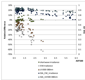
Fig.11. Comparisons between measurements and modelling (Relative Difference=Measurement/Modelling-1%) for shortwave irradiance, UV300-380nm and EW irradiance (left axis) and the retrievals of SSA for EW irradiance and UV300-380nm (right axis). See the details in the text.
