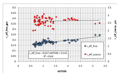
Fig.7. Changes in effective radii of fine (left axis) and coarse (right axis) aerosol modes versus aerosol content (AOT500) during the fire conditions. The regression equation is given for fine mode particles.
