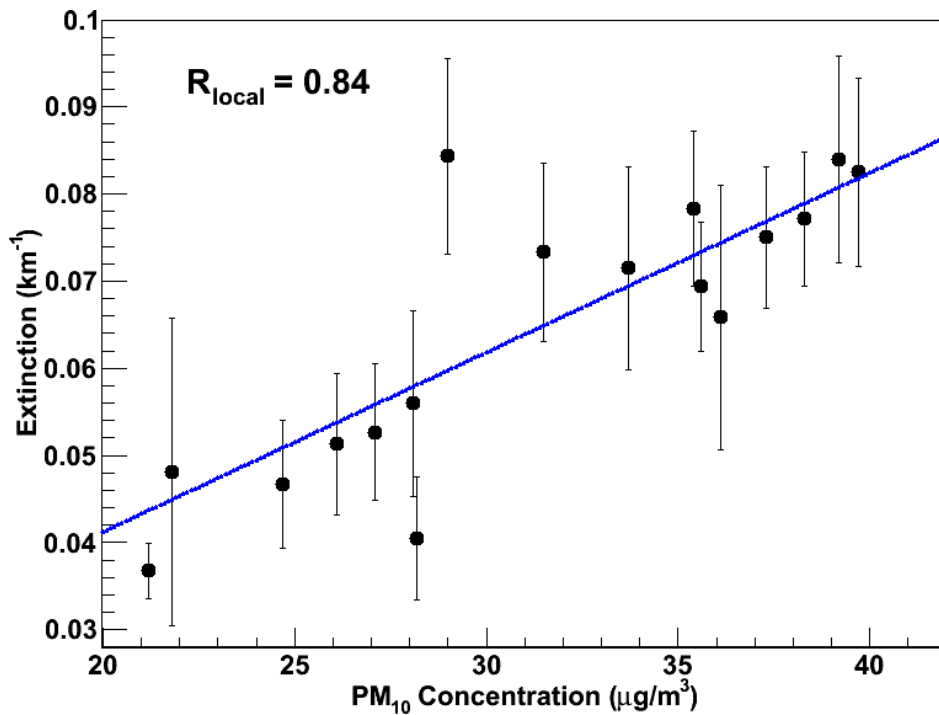
Fig. 1. The correlation between the lidar derived extinction and PM10 concentration. The extinction was obtained from a localized area with a radius R \leq 300 m directly above the PM10 measuring site.
