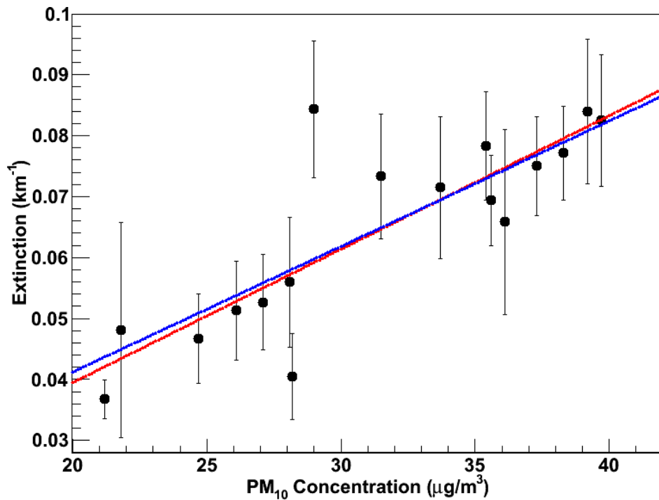
Fig. 3. In both constrained and unconstrained cases the correlation between the PM 10 concentration and the extinction was found to be 0.84. The constant term in the unconstrained fit is consistent with zero.
