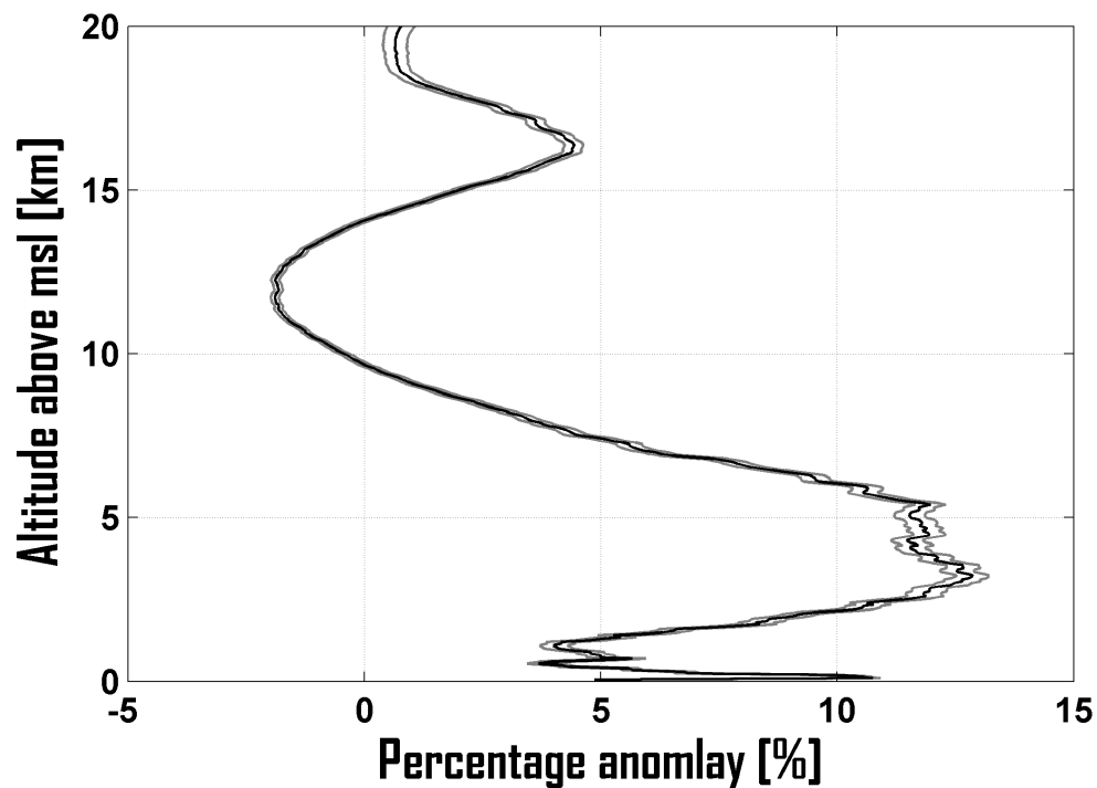
Fig. 2. Averaged bending angle anomaly profile for 1194 TC cases from 1995 to 2009 (black line) \pm with the standard deviation of the mean (grey lines)
