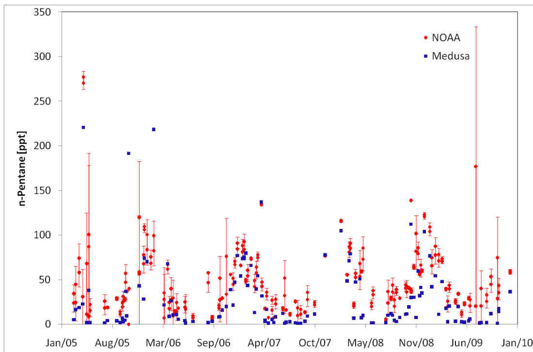
Fig. 7. Comparison of n-Pentane in Mace Head NOAA flask samples and Medusa hydrocarbon data collected within 1 hour of the flask sampling time from 2005 and 2009.
