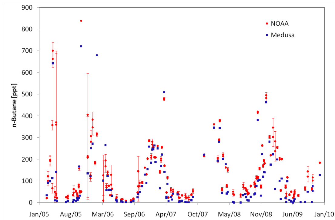
Fig. 5. Comparison of n-Butane in Mace Head NOAA flask samples and Medusa hydrocarbon data collected within 1 hour of the flask sampling time from 2005 and 2009.
