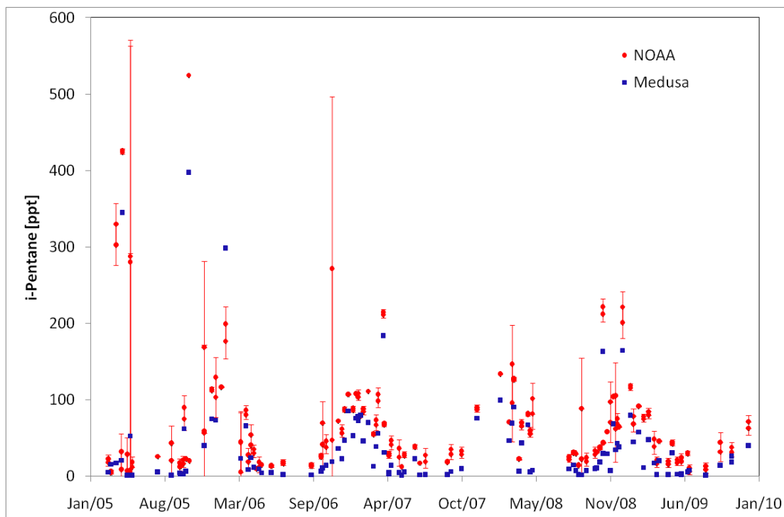
Fig. 6. Comparison of i-Pentane in Mace Head NOAA flask samples and Medusa hydrocarbon data collected within 1 hour of the flask sampling time from 2005 and 2009.
