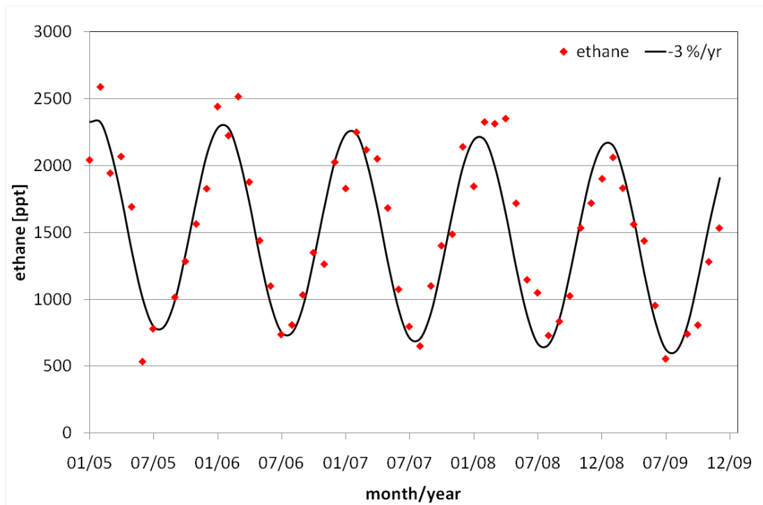
Fig. 1. Harmonic fit of monthly averaged data from European air masses arriving at Mace Head.
