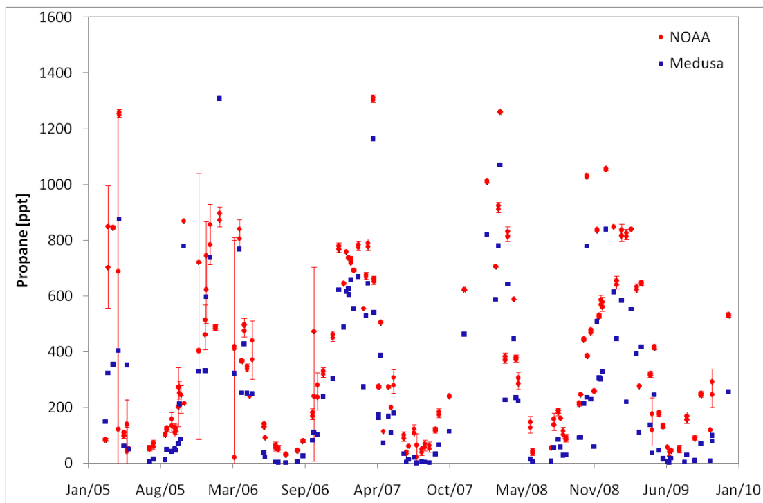
Fig. 3. Comparison of propane in Mace Head NOAA flask samples and Medusa hydrocarbon data collected within 1 hour of the flask sampling time from 2005 and 2009.
