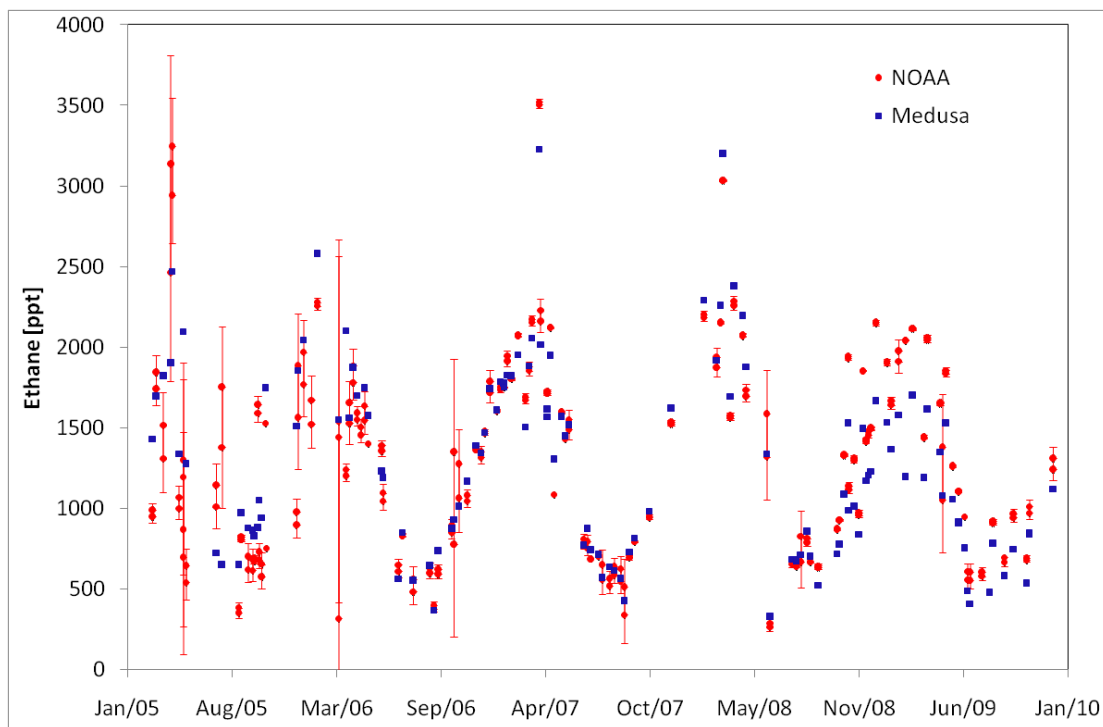
Fig. 2. Comparison of ethane in Mace Head NOAA flask samples and Medusa hydrocarbon data collected within 1 hour of the flask sampling time from 2005 and 2009.
