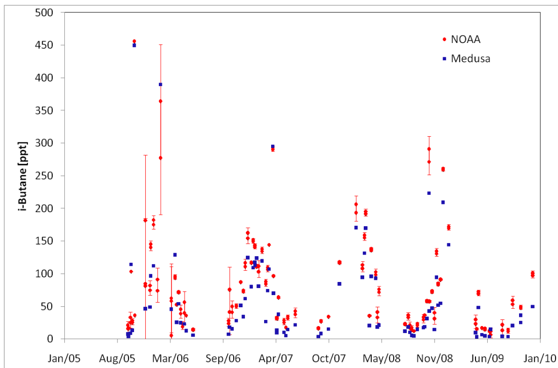
Fig. 4. Comparison of i-Butane in Mace Head NOAA flask samples and Medusa hydrocarbon data collected within 1 hour of the flask sampling time from 2005 and 2009.
