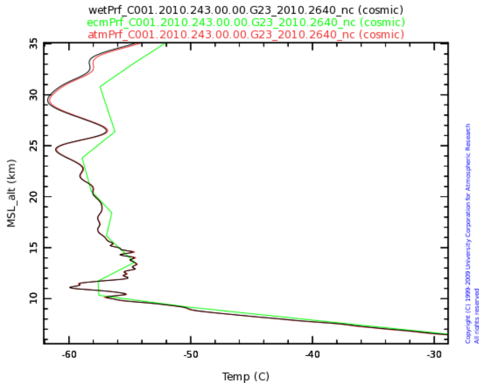
Fig. 1. Temperature profile comparison from different products.
