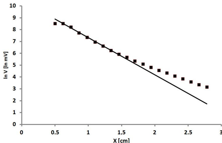
Fig. 6. Example of a calibration diagram, with the measuring points (squares) of the logarithmic output signal in relation to the path length X for nearly constant partial density of water vapour and oxygen (note that this appears similar to the original calibration curve from Campbell Sci., except that there the abscissa represents the absolute humidity for constant path length), and the regression line in the nearly log-linear part of the response function, device KH20 No. 1649, Zwickau 14 July 2011, \rho_w = 7.8 \text{ g m}^{-3} , \rho_o = 241 \text{ g m}^{-3} .
