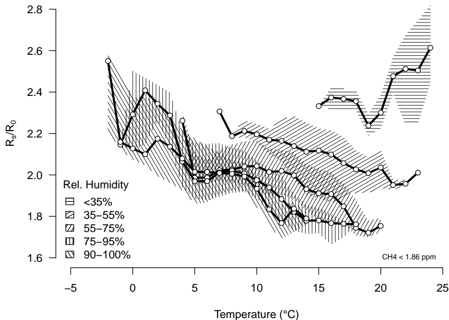
Fig. 3. Observed sensor sensitivity to ambient temperature and relative humidity at \text{CH}_4 concentrations < 1.86 ppm during the full 2011 field season at Toolik Lake. At relative humidities \geq 35\% the sensor resistance ratio follows the expected curves in Fig. 1b with an offset, but if the air is too dry (relative humidity < 35\% ) the sensor does not provide reliable data that could be used to quantify \text{CH}_4 concentrations. Each curve and shaded area shows the binned median and interquartile range, respectively, of the selected range of relative humidities (see legend). Temperature bins were chosen 2^\circ\text{C} wide with 50\% overlap.
