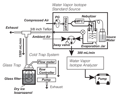
Fig. 1. Experimental setup for (a) laboratory test and (b) field evaluation.
