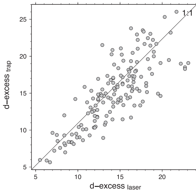
Fig. 11. Comparison of d -excess in water vapor using the cold trap and WVIA methods. The WVIA-measured d -excess values were derived from corrected and calibrated \delta D and \delta^{18}O values and then time-averaged values were calculated.
