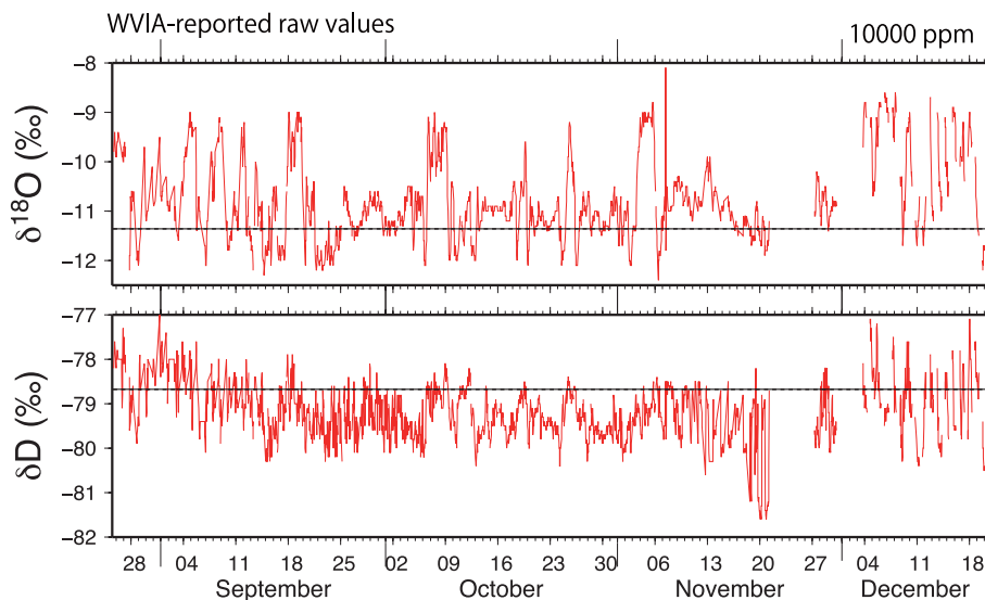
Fig. 4. Time series of uncalibrated \delta D and \delta^{18}O values of a single water standard ( \delta D = -78\% and \delta^{18}O = -11.3\% ) measured using the WVIA from late August through mid-December, 2011. The data represent the uncorrected and uncalibrated \delta D and \delta^{18}O values recorded by the WVIA and show the amount of instrument drift over the multimonth period.
