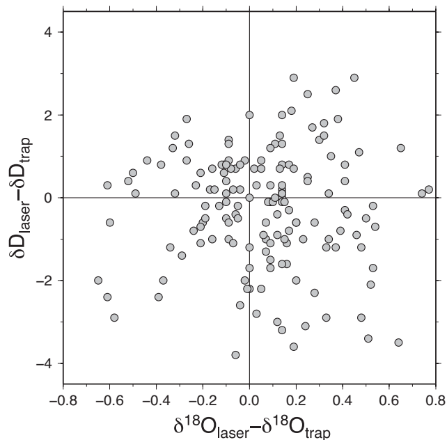
Fig. 10. Comparison of \delta\text{D} and \delta^{18}\text{O} of water vapor collected via the cold trap method and directly measured using the WVIA. For improved comparison, the time-averaged isotopic values of WVIA measurements during vapor trapping periods are plotted.
