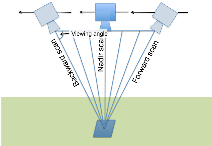
Fig. 1. Schematics of a generic multi-angle viewing mode using the satellite motion in low earth orbit instead of multiple spectrometers to record the same scene at various angles (similar to the OCO-2 target mode).
