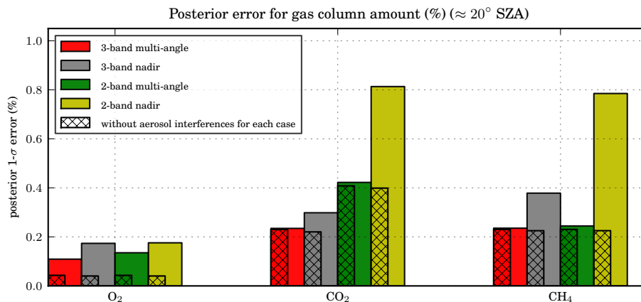
Fig. 7. Posterior error estimates ( 1-\sigma ) of trace gas total column amount in %. Summer case (Table 2), OCO-2 spectral resolutions and SNR = 200 for each spectrum was assumed.
