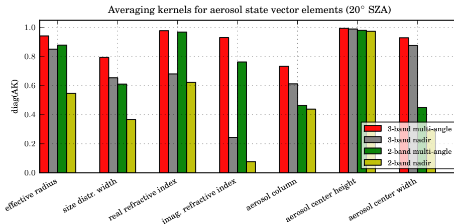
Fig. 3. Averaging kernel diagonal elements related to aerosols in the low solar zenith angle case ( \approx 20^\circ ). FWHM = 0.04 nm, 0.075 nm and 0.1 nm in the O_2 A-band, weak CO_2/CH_4 band and strong CO_2 band, respectively; 2.5 spectral samples per FWHM, SNR = 200 for each band.
