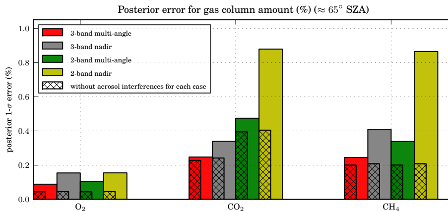
Fig. 8. Posterior error estimates ( 1-\sigma ) of trace gas total column amount in %. Winter case (Table 2), OCO-2 spectral resolutions and SNR = 200 for each spectrum was assumed.
