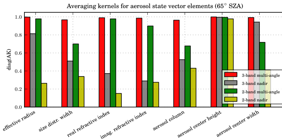
Fig. 4. Averaging kernel diagonal elements related to aerosols in the high solar zenith angle case ( \approx 65^\circ ). Otherwise, same as Fig. 3.
