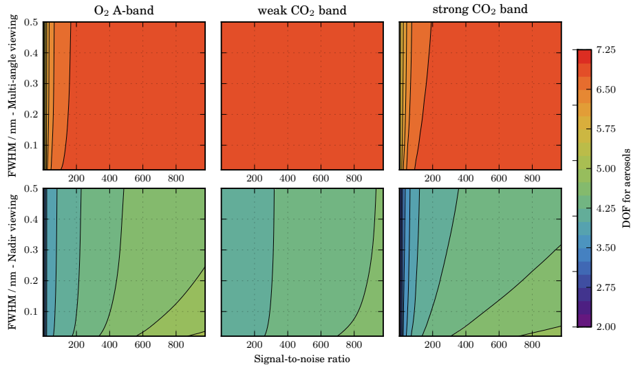
Fig. 6. High solar zenith angle case. Otherwise like Fig. 5. Note that the theoretically maximum of DOF in our setup is 7, i.e., the total amount of aerosol state vector elements.
