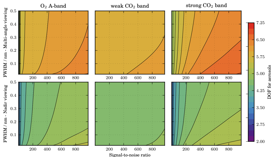
Fig. 5. Low solar zenith angle case: contour plot visualization of the degrees of freedom (DOF) for aerosol state vector elements as a function of signal-to-noise ratio (SNR) and spectral resolution (in full width at half maximum (FWHM) of the instrument line-shape (ILS)). Note that oversampling of the ILS increases with FWHM in order to keep the amount of detector pixels used in the retrieval constant. In each panel, specifications of only one spectrometer (left: O 2 A-band, middle: weak CO 2 band, right: strong CO 2 band) were changed while the remaining two were kept at nominal levels: FWHM = (0.04 nm; 0.075 nm; 0.1 nm), SNR = (150; 150; 150) for the O 2 A-band, weak CO 2 band and strong CO 2 band, respectively. The top row shows the multi-angle case, the bottom row the pure Nadir viewing case. Black lines indicate a 0.25 unit change in DOF.
