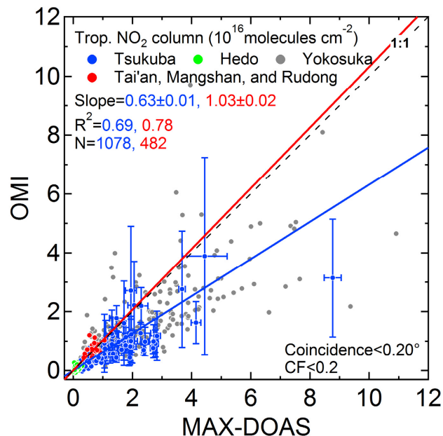
Fig. 2. Correlations between tropospheric \text{NO}_2 VCDs ( 10^{16} molecules \text{cm}^{-2} ) from OMI and MAX-DOAS observations at a coincidence criterion ( x ) of 0.20^\circ . Comparisons over Tsukuba, Hedo, and Yokosuka are shown in blue, green, and gray, respectively, and campaign-based short-term observations in China are shown in red. Error bars for both OMI and MAX-DOAS data are shown only for comparisons over Tsukuba at MAX-DOAS \text{NO}_2 VCDs larger than 1 \times 10^{16} molecules \text{cm}^{-2} , for clarity. Linear regression analysis has been performed for the respective cases 1 (Tokyo case; blue) and 2 (Chinese case; red), where the slopes of their regression lines are constrained mainly by comparisons made around Tokyo (Tsukuba and Yokosuka) and at China sites (Tai'an, Mangshan, Rudong), respectively. Hedo data are used in both regression analyses but do not constrain the slope much, since the comparisons at other sites are made over a wide range of \text{NO}_2 VCD values. For each case, the slope, correlation coefficient ( R^2 ), and number of data points ( N ) are given in the plot.
