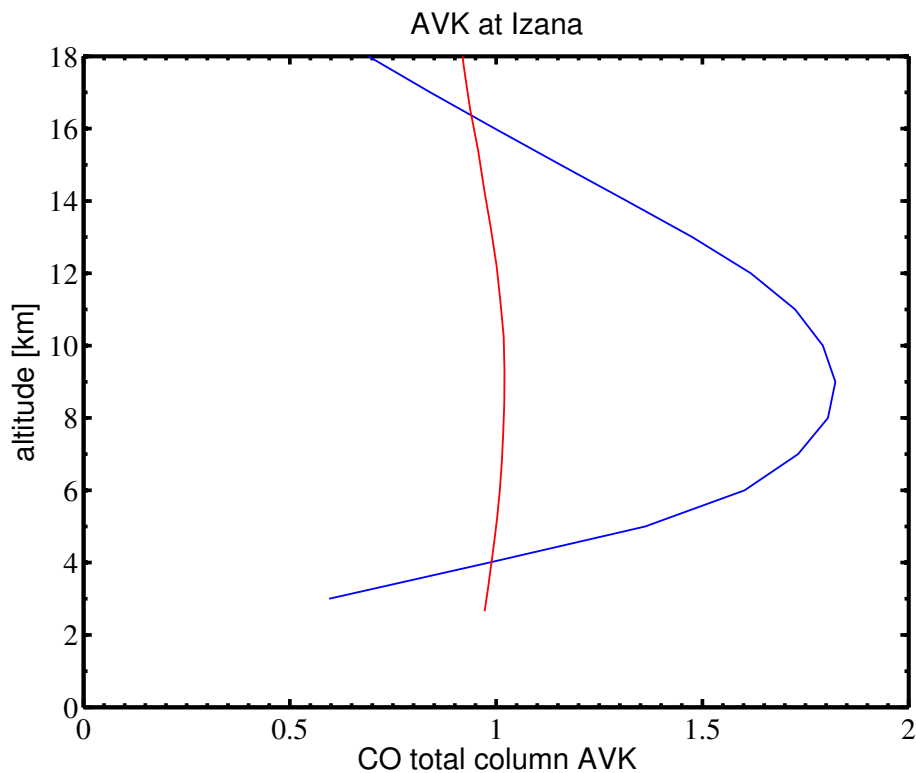
Fig. 2. Mean ground-based FTIR averaging kernels (red) compared to the mean IASI averaging kernel (blue) for Izaña. The averaging kernels are shown for altitudes above the station (2367 m).
