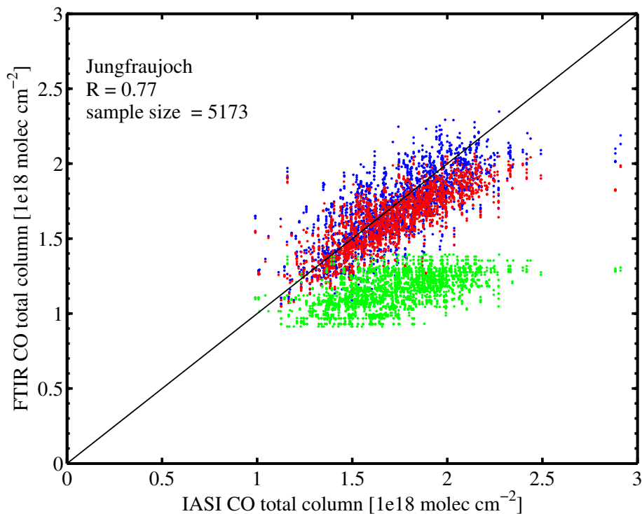
Fig. 3. FTIR CO total columns against the IASI CO for the uncorrected, unsmoothed columns (green), the altitude adjusted (red) and altitude adjusted, smoothed columns (blue) for Jungfraujoch. The correlation coefficient of the comparison between the altitude adjusted, smoothed FTIR CO and IASI CO (blue) is shown. For clarity, only every second data point is plotted.
