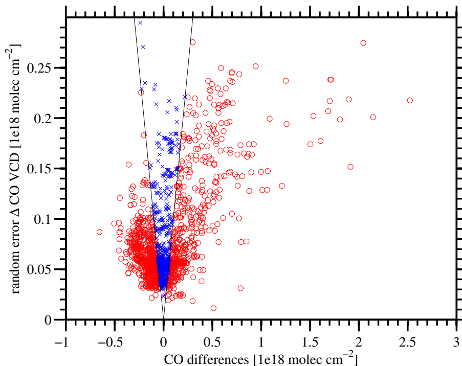
Fig. 6. Carbon monoxide random error of the differences against differences of the IASI-FTIR total column for the quality filtered data for Kiruna. For the values indicated in blue (red) the absolute values of the differences are smaller (larger) than the random errors (VCD = vertical column density).
