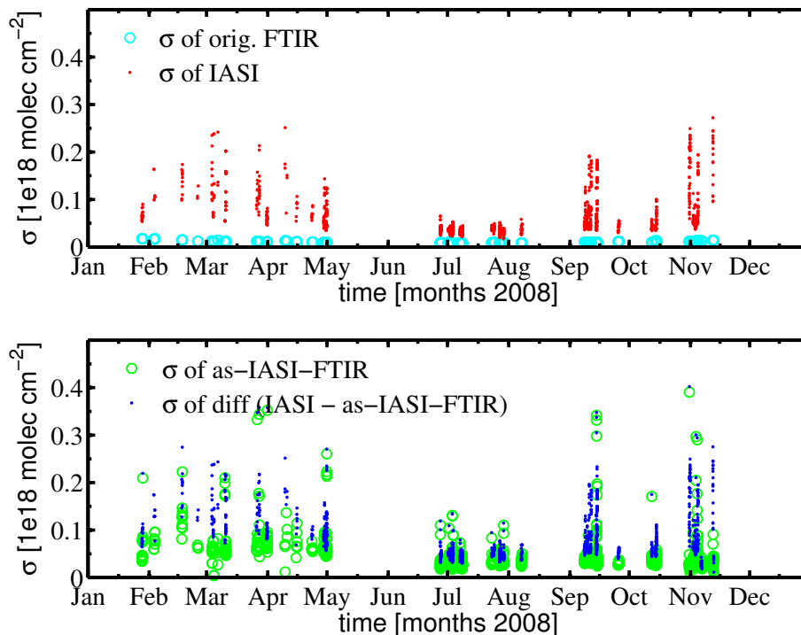
Fig. 5. Carbon monoxide random errors, \sigma , for the quality filtered data against time at Kiruna. Shown are the errors for the original FTIR total columns (cyan open circles), the IASI total columns (red dots), the as-IASI-FTIR total columns (green open circles) and the random errors of the differences between IASI and as-IASI-FTIR total columns (blue dots).
