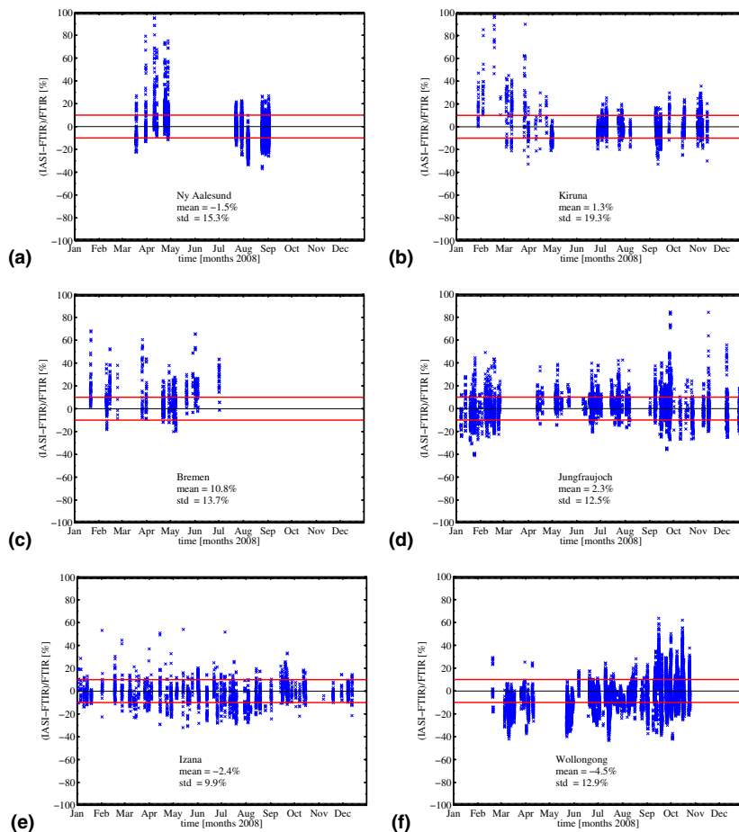
Fig. 4. Relative differences of the smoothed and altitude corrected FTIR CO total column and the IASI CO total column of all the comparison pairs for (a) Ny Ålesund, (b) Kiruna, (c) Bremen, (d) Jungfraujoch, (e) Izaña and (f) Wollongong. The red lines indicate \pm 10\% difference.
