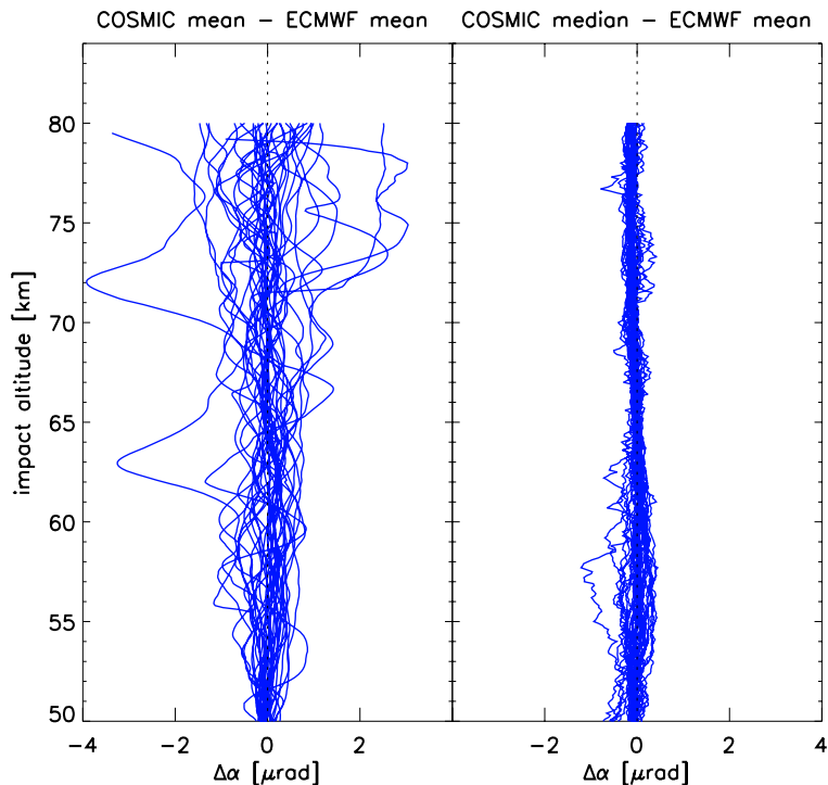
Fig. 2. Mean bending angle profiles (left panel), and median bending angle profiles (right panel), for January 2011 within 5-degree latitudinal bins, after subtraction of ECMWF analysis data mapped to bending angle space. Above 50 to 60 km, the lower variability of the median profiles indicates that they provide a more robust measure of the central value of the bending angle distribution.
