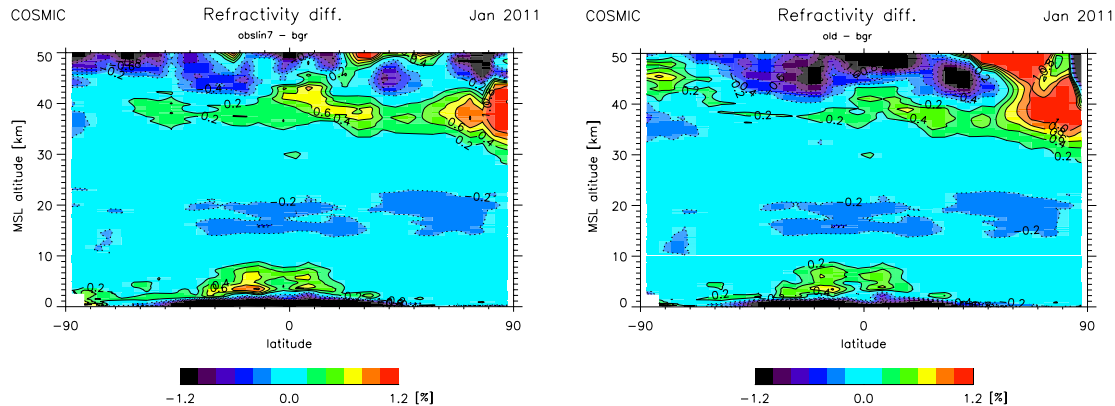
Fig. 5. Relative differences between monthly mean refractivity from COSMIC data and from collocated ECMWF data, using average-profile inversion (left panel) and single-profile inversion including statistical optimization (right panel). Data for January 2011.
