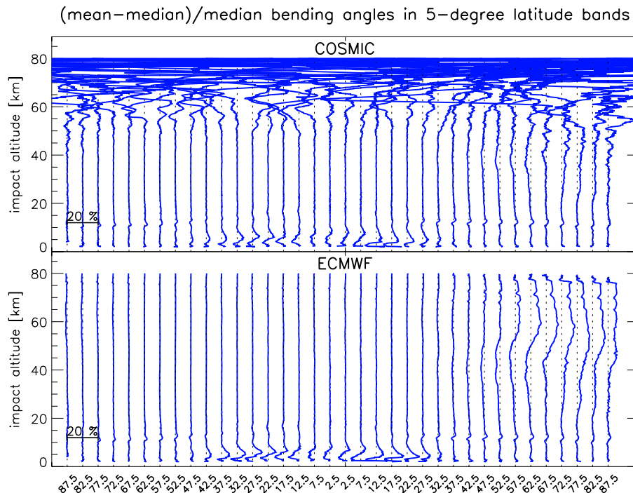
Fig. 3. Relative differences between bending angle means and medians for observed COSMIC data (upper panel), and collocated ECMWF analysis data (lower panel). Data are from January 2011 binned into 5-degree latitude bands. In the troposphere and lower stratosphere, the observed mean–median differences are very similar to the collocated ECMWF data, indicating a real neutral-atmosphere origin. In contrast, the observed mean–median differences above 50 to 60 km are strongly influenced by large measurement errors.
