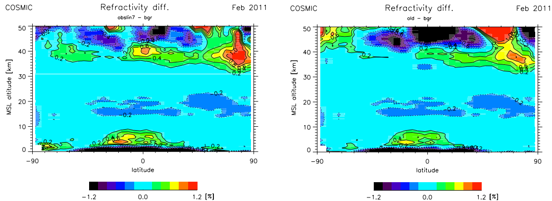
Fig. 6. Relative differences between monthly mean refractivity from COSMIC data and from collocated ECMWF data, using average-profile inversion (left panel) and single-profile inversion including statistical optimization (right panel). Data for February 2011.
