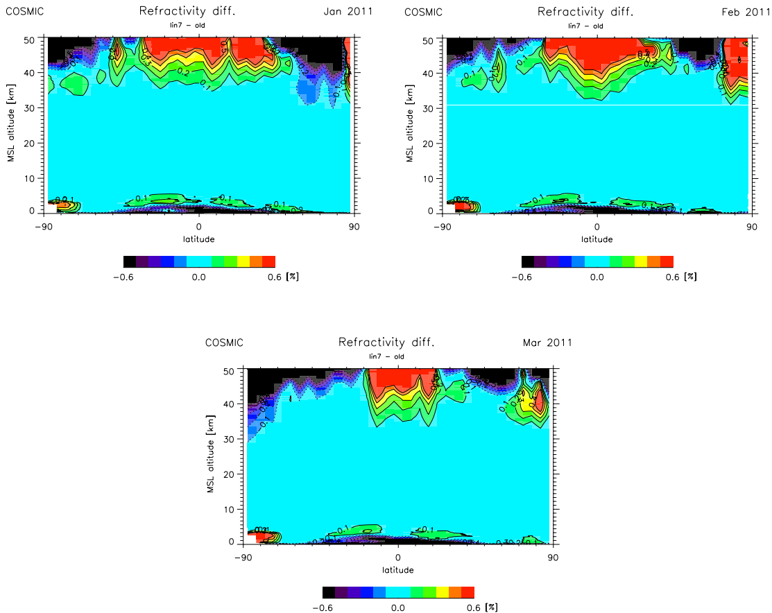
Fig. 4. Relative differences between monthly mean refractivities obtained by average-profile inversion and single-profile inversion. Data for the first three months of 2011.
