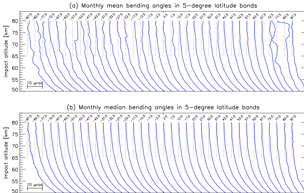
Fig. 1. (a) Observed bending angle means, and (b) observed bending angle medians, for COSMIC data from January 2011 within 5-degree latitudinal bins. Above 55 to 60 km an increasing impact of measurement errors shows up as large-scale wiggles in the means, occasionally leading to negative bending angles. The medians do not show the corresponding wiggles, although higher-frequency variations are evident.
