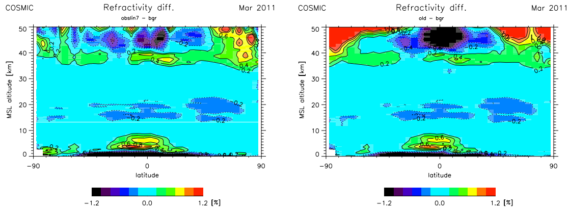
Fig. 7. Relative differences between monthly mean refractivity from COSMIC data and from collocated ECMWF data, using average-profile inversion (left panel) and single-profile inversion including statistical optimization (right panel). Data for March 2011.
