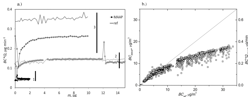
Fig. 2. (a) Examples of the artifact temporal response. Symbol lines indicate data from the high flow rate MAAP, and solid lines data from the reference MAAP. Three regimes of different artifact behavior are indicated. See text for details. (b) Comparison of the low flow rate reference ( BC_{ref} ) and high flow rate ( BC_{MAAP} ) BC concentrations.
