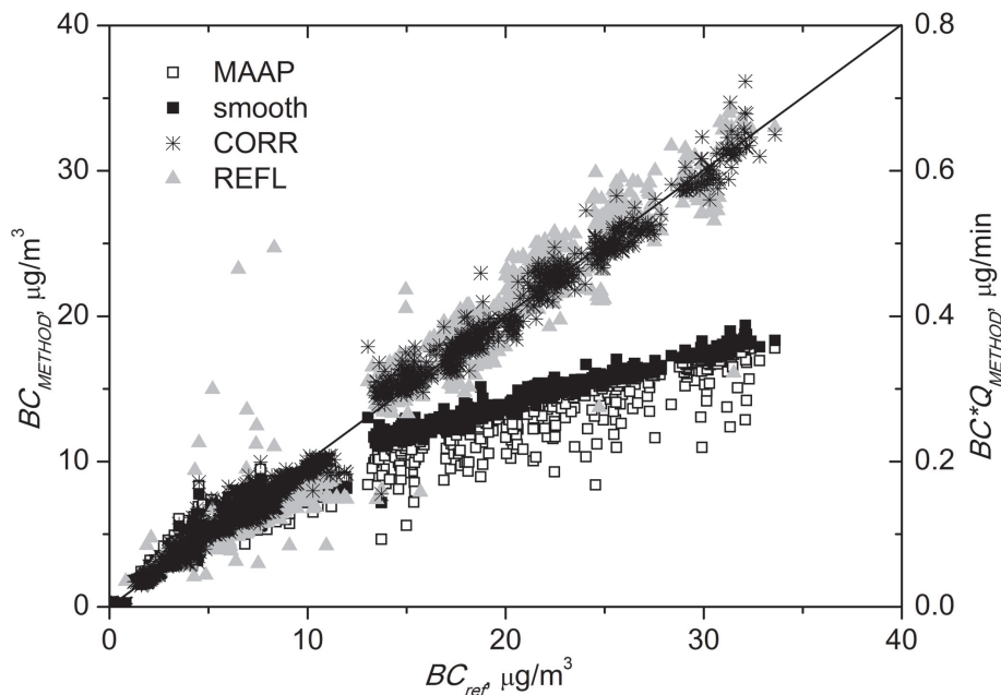
Fig. 3. High flow rate MAAP BC concentrations as a function of the reference (low flow rate) MAAP concentrations. BC_{\text{MAAP}} is the original signal, BC_{\text{smooth}} is the smoothed signal without an overall concentration correction. BC_{\text{CORR}} is the smoothed signal with the overall concentration correction. BC_{\text{REFL}} is the original signal determined with the reflectance method. The 1 : 1 ratio line is also shown.
