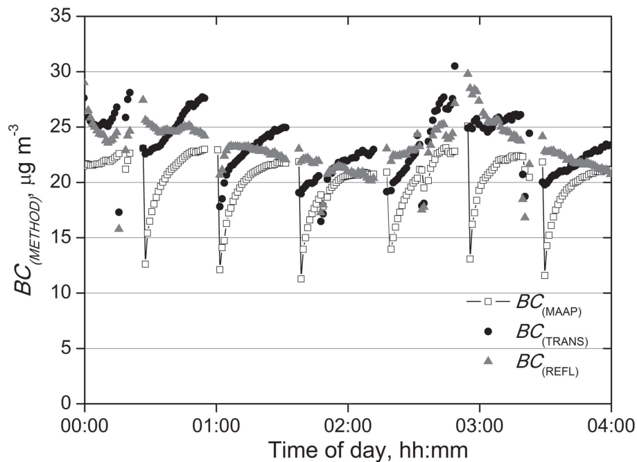
Fig. 1. Comparison of BC measured with the MAAP by multi-angle photometry BC_{\text{MAAP}} , transmission BC_{\text{TRANS}} and reflectance BC_{\text{REFL}} methods during a high concentration episode in Gual Pahari, India 12 August 2009.
