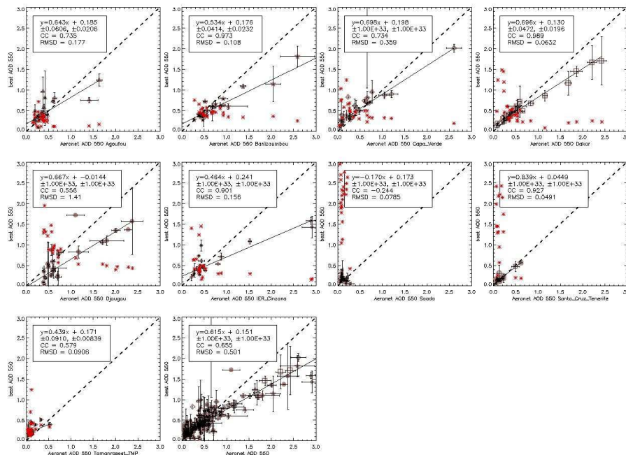
Fig. 11. Combined daily AOD vs. AERONET. Equivalent of Fig. 4 but obtained considering the combined AOD instead of a single satellite dataset. Different locations are shown in different plots and are represented by different symbols, as with Fig. 3. The red stars represent two times the AERONET Ångström coefficient (between 440 and 870 nm). The final plots show all the coincidences.
