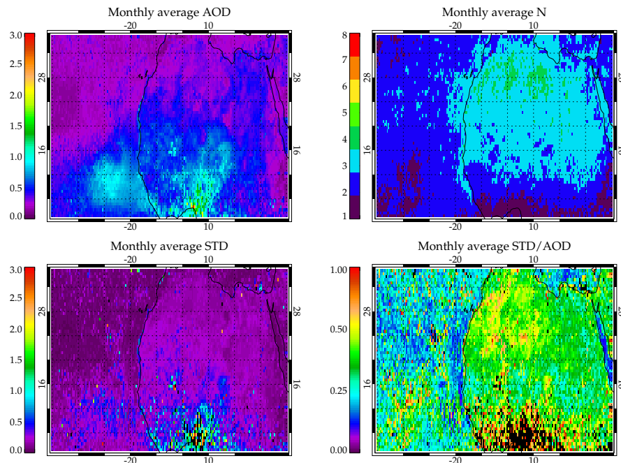
Fig. 13. Monthly average of AOD (top left), number N of instruments considered (top right), standard deviation (bottom left) and ratio between standard deviation over AOD (bottom right). Values in black are higher than the maximum of the colourbar.
