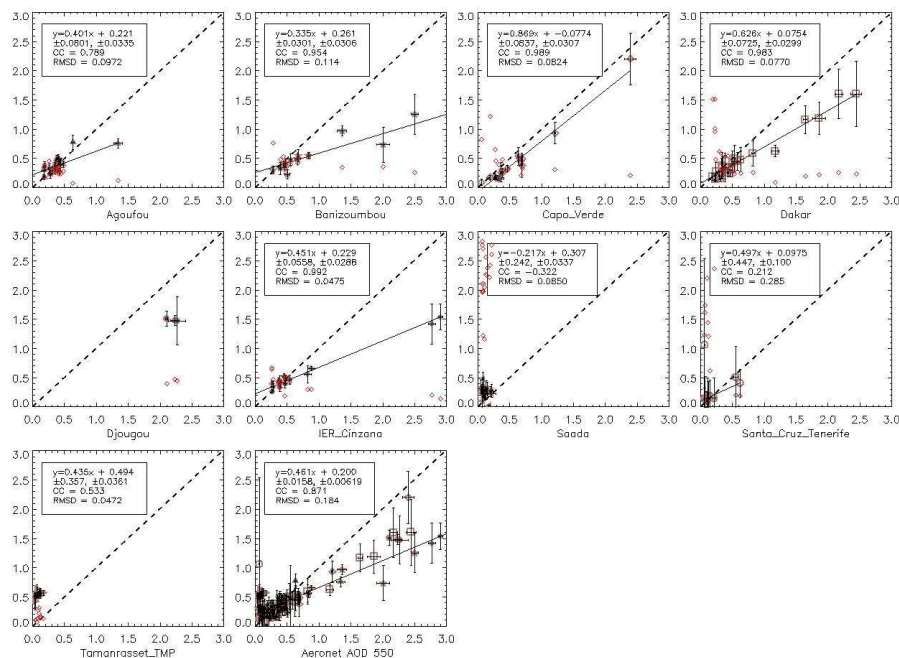
Fig. 4. Example of a scatter plot between AERONET data (x) and satellite (y) for SEVIRI-ORAC. The black/brown symbols are satellite datasets (y) vs. AERONET AOD (x). Different locations are represented by different symbols, as with Fig. 3. The red stars represent two times the AERONET Ångström coefficient (between 440 and 870 nm). The final plots show all the coincidences. In every scatter plot with more than four coincidences there are captions indicating the best linear fit (angular coefficients, y intercept and associated errors), the correlation coefficient (CC) and the root mean square differences (RMSD).
