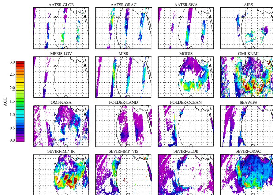
Fig. 1. Image of AOD of the different datasets corresponding to 8 March 2006.
