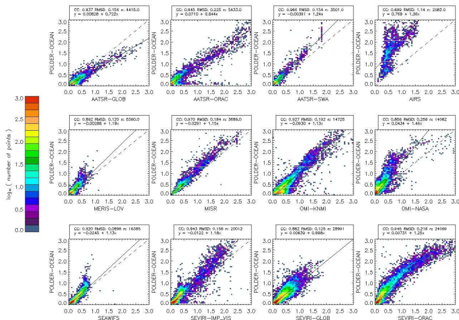
Fig. 7. Example of scatter plots over ocean, POLDER-OC vs. other datasets. In every scatter plot there is a caption: the first line indicates the correlation coefficient (CC), the root mean square differences (RMSD) and the number of coincidences ( n ); the second line presents the best linear fit.
