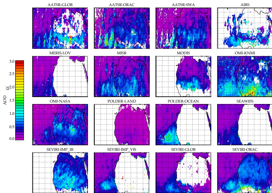
Fig. 2. Image of monthly mean AOD of the different datasets for March 2006.
