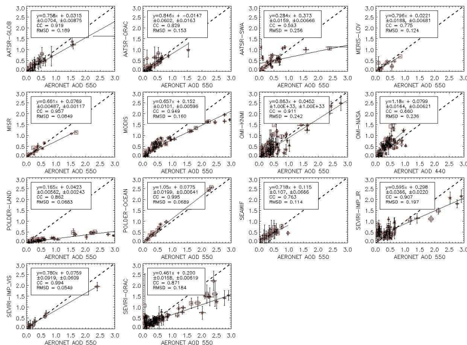
Fig. 5. Scatter plots, satellite datasets AOD (y) vs. AERONET AOD (x), for all the available coincidences. Different locations are represented by different symbols, as defined in Fig. 3. In every scatter plot there are captions indicating the best linear fit (angular coefficients, y intercept and associated errors), the correlation coefficient (CC) and the root mean square differences (RMSD).
