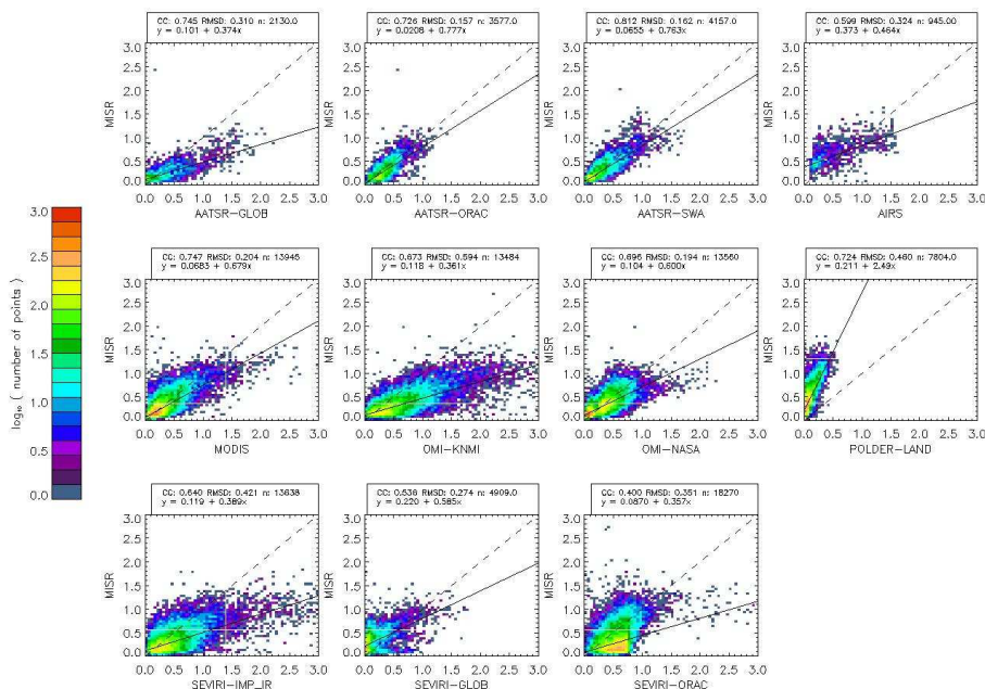
Fig. 6. Example of comparison over land, MISR vs. other datasets. In every scatter plot there is a caption: the first line indicates the correlation coefficient (CC), the root mean square differences (RMSD) and the number of coincidences ( n ); the second line presents the best linear fit.
