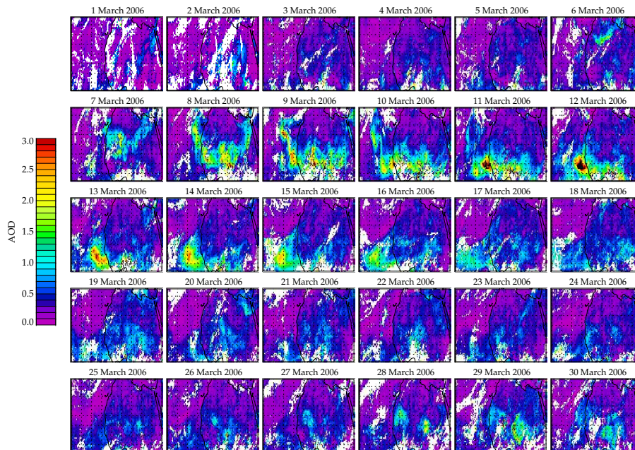
Fig. 10. Combined daily AOD for the first 30 days of March 2006.
