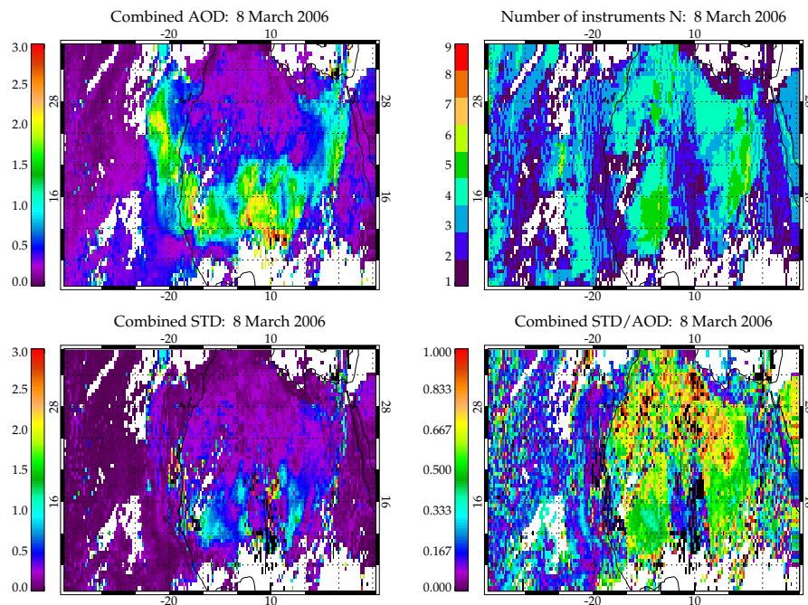
Fig. 12. Daily map for 8 March 2006 of the combined AOD (top left), the number N of instruments considered for every box (top right), standard deviation STD (bottom left) and ratio between standard deviation and aerosol optical depth STD/AOD (bottom right).
