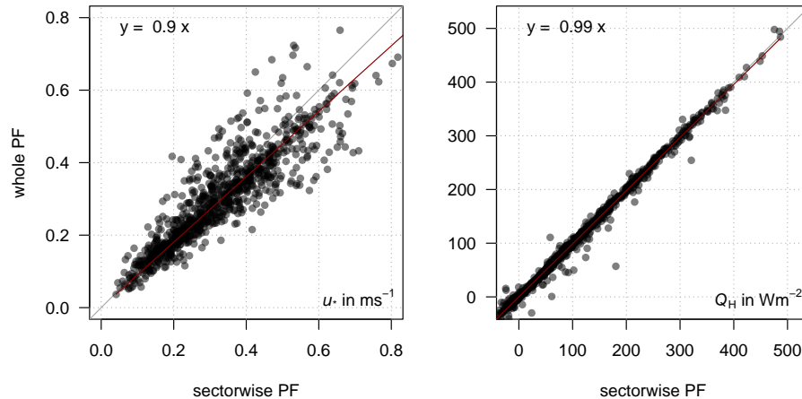
Fig. 5. Comparison of the friction velocity (left) and the sensible heat flux (right) with planar fit rotation for all wind directions and for sector wise planar-fit rotation and data quality 1–3 (data set A, DAT 600).
