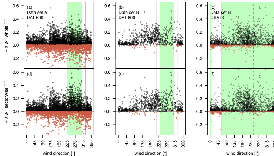
Fig. 4. Covariance -\overline{u'w'} and its dependency on the wind direction for rotated data and high data quality (flag 1–3 according to Foken et al., 2004); The upper row displays -\overline{u'w'} , data rotated for the whole period (a–c), the lower row -\overline{u'w'} , data rotated sectorwise (d–f); columns represent DAT 600, data set A on the left (a, d), DAT 600, data set B in the middle (b, e) and CSAT3, data set B on the right (c, f). The green sector is the undisturbed sector and the red points indicate data with -\overline{u'w'} < 0 ; dashed lines for CSAT3 indicate the front sector, which is rotated separately.
