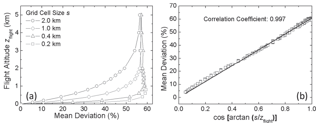
Fig. 7. (a) Vertical profile of the mean albedo deviation \bar{\Delta} for different horizontal resolutions. (b) Correlation of mean albedo deviation and \cos \theta with \theta = \arctan(s/z_{\text{flight}}) .
