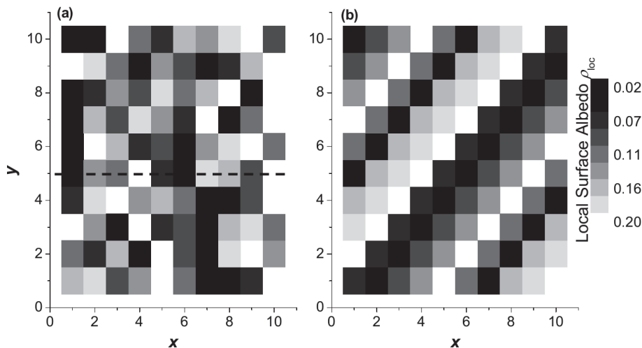
Fig. 5. Albedo maps at 450 nm wavelength with different distributions: (a) randomly and (b) systematically with variable grid size between 0.1 km and 2 km. The dashed line marks the position of a cross-section through the model domain.
