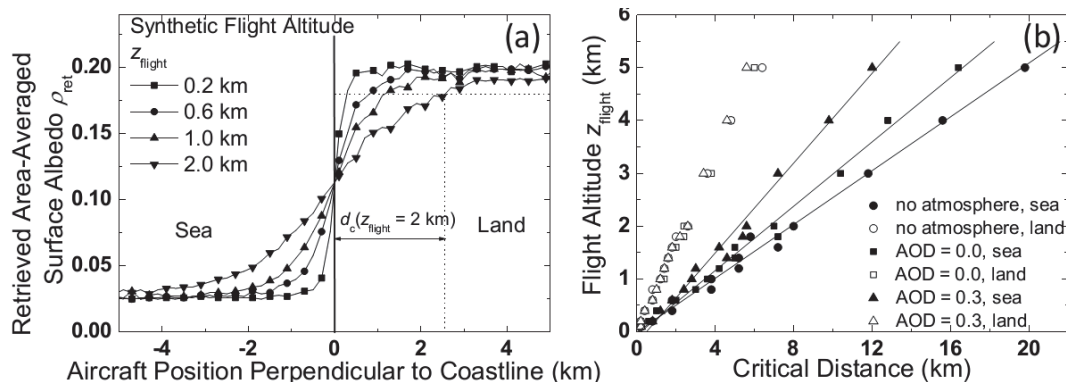
Fig. 2. (a) Cross-section of retrieved surface albedo \rho_{\text{ret}} across the coastline (solar zenith angle \theta_0 = 30^\circ , aerosol optical depth AOD = 0.3). (b) Critical distance to coastline dependent on flight altitude ( \theta_0 = 30^\circ ).
