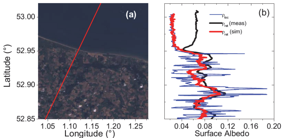
Fig. 8. (a) Landsat image and flight track of the studied area over East Anglia, (b) Retrieved area-averaged surface albedo from simulations and local surface albedo taken from Landsat at 660 nm along the flight leg. Additionally, the retrieved area-averaged surface albedo from aircraft measurements is shown.
