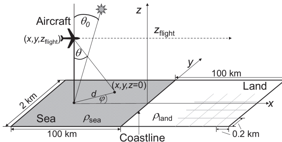
Fig. 1. Synthetic flight geometry with aircraft flying in altitude z_{\text{flight}} . The aircraft flies perpendicular to the coastline at constant altitude.
