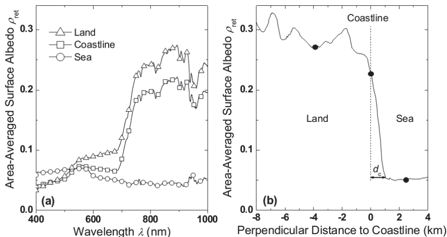
Fig. 4. (a) Measured spectra of area-averaged surface albedo \rho_{\text{ret}} for land, sea, and coastline. (b) \rho_{\text{ret}} for 870 nm wavelength along the coastal overflight. The black dots mark the measurement points of the spectra from (a).
