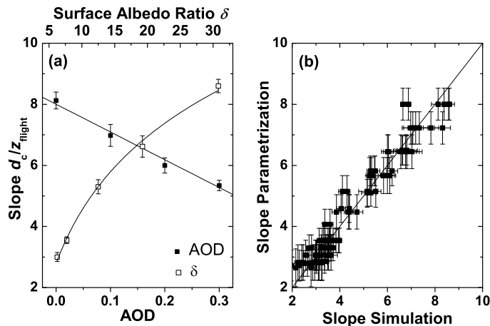
Fig. 3. (a) Slope d_c/z_{\text{flight}} as a function of aerosol optical depth ( \theta_0 = 50^\circ , \delta = 30.8 ), and surface albedo ratio \delta = \rho_{\text{land}}/\rho_{\text{sea}} ( \theta_0 = 30^\circ , AOD = 0.1). (b) Relationship of the slopes derived from the radiative transfer simulation and the parameterized slopes. Additionally, the one-to-one line is plotted.
