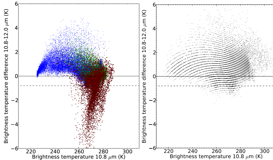
Fig. 6. Left panel: the MYSTIC simulated 10.8\mu\text{m} brightness temperature versus the 10.8\text{--}12.0\mu\text{m} brightness temperature difference. Blue, green and red points indicate pixels with ice, water and ash clouds as the uppermost cloud. The dashed horizontal line indicates the ash limit cut-off. Right panel: similar to left panel, but data from the SEVIRI. The line structures in the SEVIRI data are due to digitization. The Sahara desert has been excluded from both panels.
