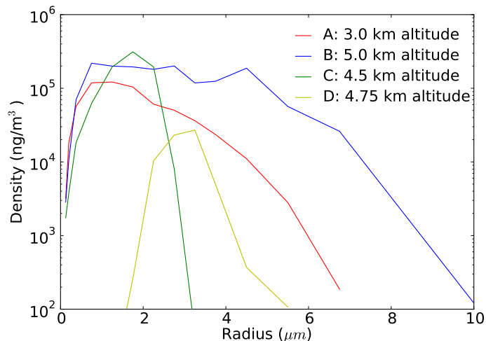
Fig. 9. The ash size distribution for locations A, B, C, and D (see upper left panel of Fig. 5 for location). The size distribution is at the altitudes of maximum ash concentrations.
