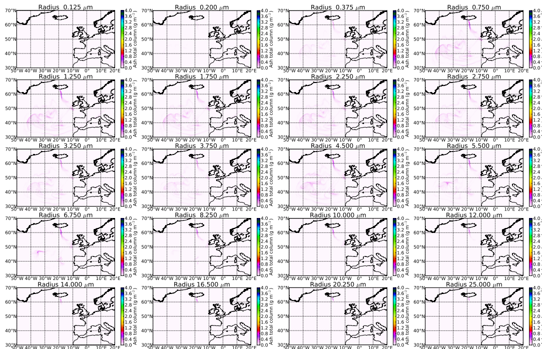
Fig. 1. The total column density of the ash for various particle radii as simulated by the FLEX-PART Lagrangian particle dispersion model for 11 May 2010 at 12:00 UTC.
