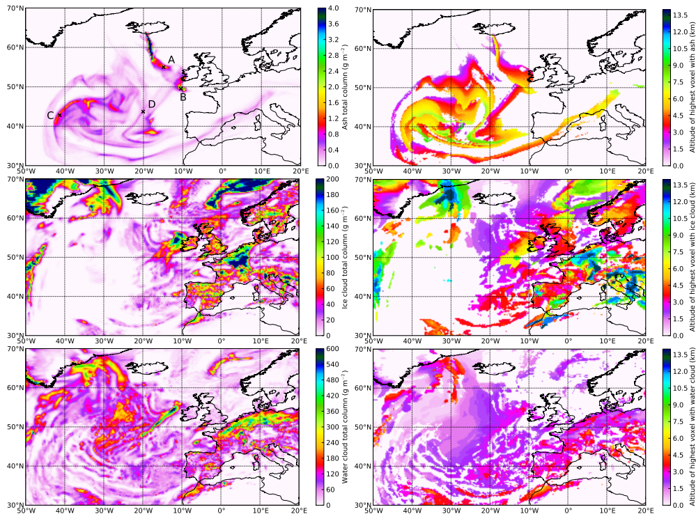
Fig. 5. Left column: the total column density of the ash as simulated by FLEXPART (top panel), and ice (middle panel) and water (bottom panel) clouds from ECMWF. Right column: the altitude of the highest voxel with ash concentration above 0.1 \text{ mg m}^{-3} (top panel), ice above 10 \text{ mg m}^{-3} (middle panel), and water above 50 \text{ mg m}^{-3} (bottom panel).
