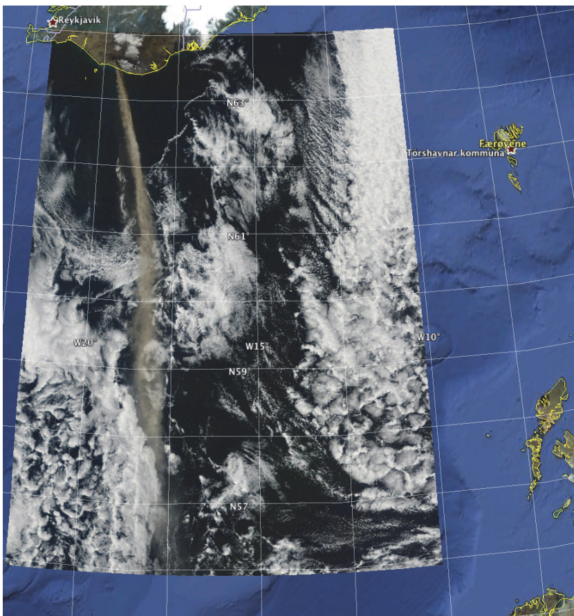
Fig. 3. MODIS true color image of the Eyjafjallajökull eruption on the 11 May 2010 at 12:15 UTC.
