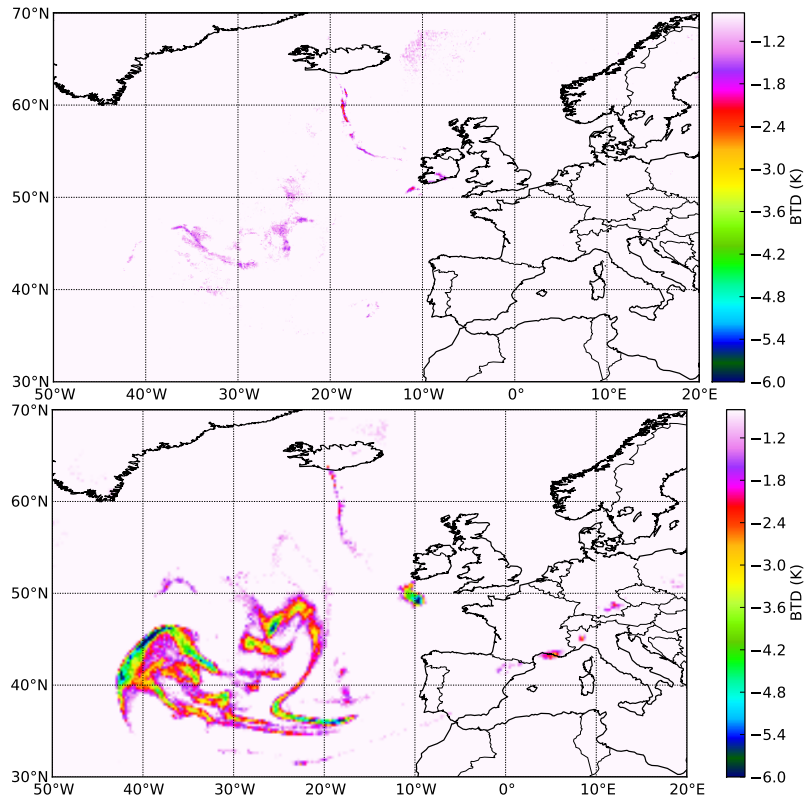
Fig. 7. Pixels identified as ash by the inverse absorption technique. Top panel: the SEVIRI 10.8–12.0 \mu\text{m} channels brightness temperature difference. Bottom panel: the simulated 10.8–12.0 \mu\text{m} channels brightness temperature difference.
