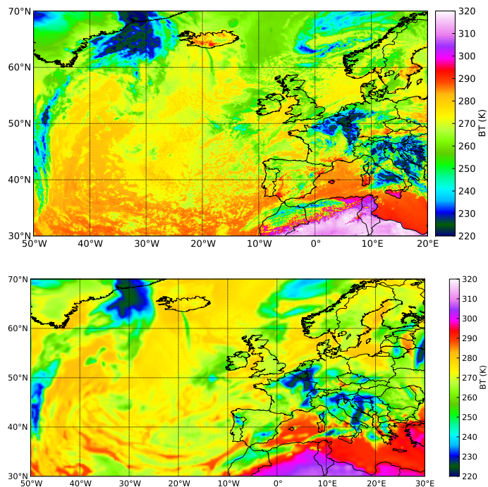
Fig. 4. top panel: brightness temperatures as measured by the 10.8 \mu\text{m} channel of the SEVIRI instrument. Bottom panel: the 10.8 \mu\text{m} as simulated by the MYSTIC radiative transfer model. The simulation includes ECMWF ice and water cloud in addition to the FLEXPART ash cloud.
