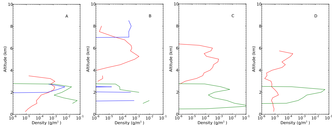
Fig. 8. The vertical ash (red), ice (blue) and water (green) cloud density profiles for the locations A (left panel), B (second panel), C (third panel) and D (right panel) in the upper left panel of Fig. 5.
