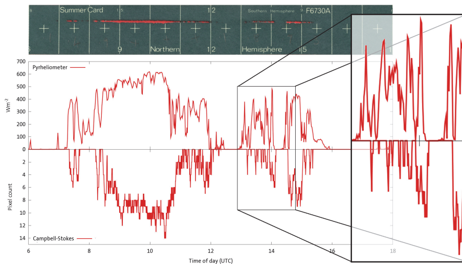
Fig. 6. Comparison between the solar data extracted from a rectified and registered Campbell-Stokes recorder card and that from the co-located pyrliometer at Lerwick. These data are for 21 April 2003. The card image has been cropped and scaled to match the time scale used for the data panels. There is a clear correlation between the data from the two sources in both time and amount despite this being only a moderately sunny day.
