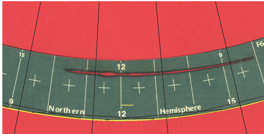
Fig. 3. Excerpt from a scan image showing how the components of the card geometry are recovered. The curved yellow line to the bottom of the card shows the detected and smoothed edge. The short yellow line in the centre shows the path of the search for the midday marker, the position of this search is deliberately performed on a portion of the card that is clear of the burn path. The straight black lines show the construction of the chords and orthogonal radial lines used to detect the centre of the card arc. The search and construction lines in this image were added to the original card image by the semi-automatic processing program operating in a mode implemented specifically to aid refinement of the extraction process. This card is from Lancaster University's Hazelrigg Field Station for 21 January 2011.
