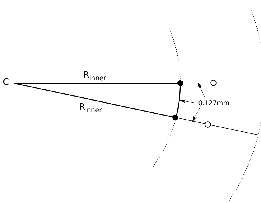
Fig. 4. Diagram showing the method of extracting pixels from an image of curved Campbell-Stokes recorder card that are required for the production of a rectified output image. The filled circles represent pixels that will form the bottom row of the rectangular output image. The empty circles represent pixels for the second from bottom row. C denotes the centre of the circular arc that is the inner edge of the card image ( R_{\text{inner}} is radius of this arc). The pitch of the selected pixels is 0.127 mm along the inner edge so that selecting other pixels on the radial lines shown will also be spaced at 0.127 mm to maintain 200 dpi pitch in the output image. The proportions of the card geometry in this diagram have been distorted to fit the page.
