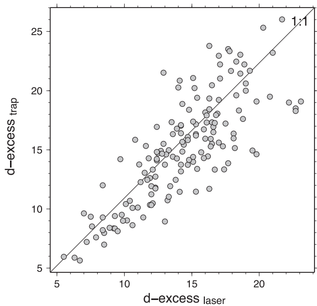
Fig. 11. Comparison of d -excess in water vapor using the cold trap and WVIA methods. The WVIA-measured d -excess values were derived from corrected and calibrated \delta\text{D} and \delta^{18}\text{O} values and then time-averaged values were calculated.
