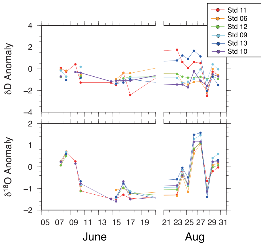
Fig. 5. Comparison of time-dependent \delta\text{D} and \delta^{18}\text{O} variations of six water standards with different isotopic compositions. Plotted values are expressed as a normalized anomaly, that is, a departure from the long-term mean for the analysis period, divided from the standard deviation during this period.
