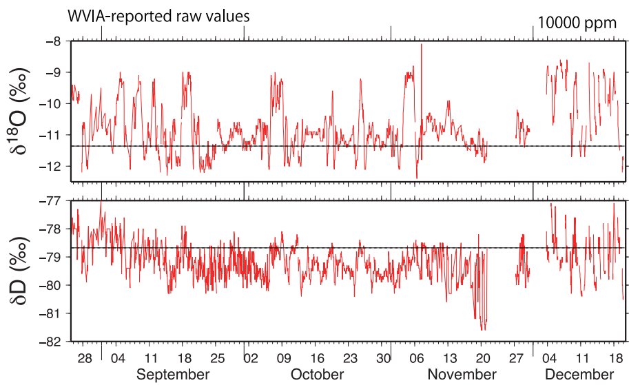
Fig. 4. Time series of uncalibrated \delta\text{D} and \delta^{18}\text{O} values of a single water standard ( \delta\text{D} = -78 ‰ and \delta^{18}\text{O} = -11.3 ‰) measured using the WVIA from late August through mid-December, 2011. The data represent the uncorrected and uncalibrated \delta\text{D} and \delta^{18}\text{O} values recorded by the WVIA and show the amount of instrument drift over the multimonth period.
