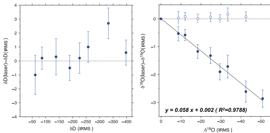
Fig. 6. The difference in WVISS based \delta D and \delta^{18}\text{O} values from known IRMS based values of each water standard (blue circle). In both figures, the x-axis represents known IRMS based SMOW/SLAP scale values. For \delta^{18}\text{O} , collected SMOW scale values are also plotted at the top of the figure (white circle).
