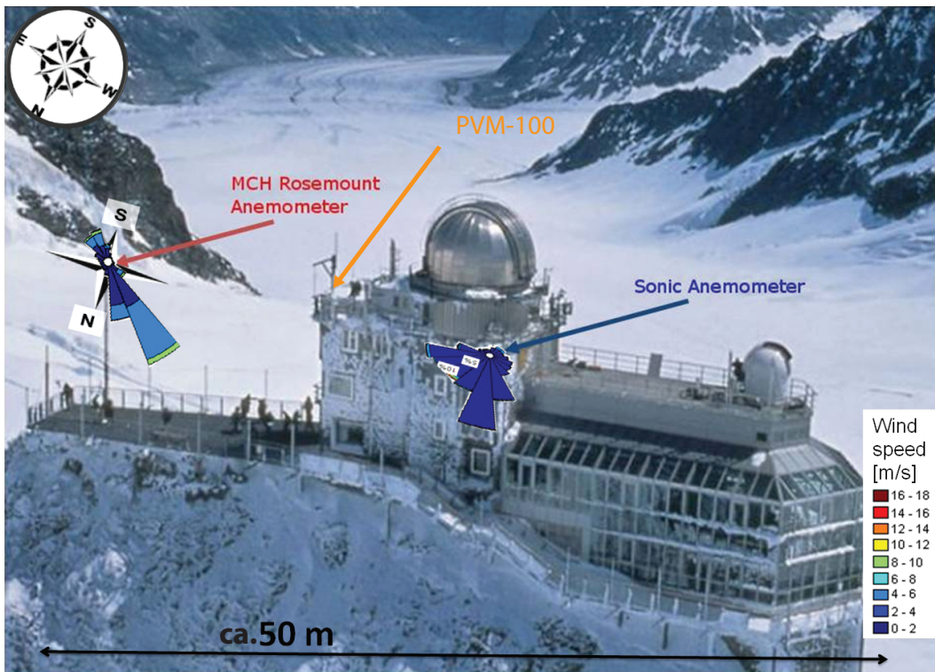
Figure 2: Photo (modified from Ketterer, 2011) showing the position of the PVM-100, the Sonic anemometer (FM-100 was employed in closed vicinity) as well as the MCH Rosemount anemometer permanently deployed by MeteoSwiss. The corresponding wind roses during CLACE 2010 are depicted as well.
