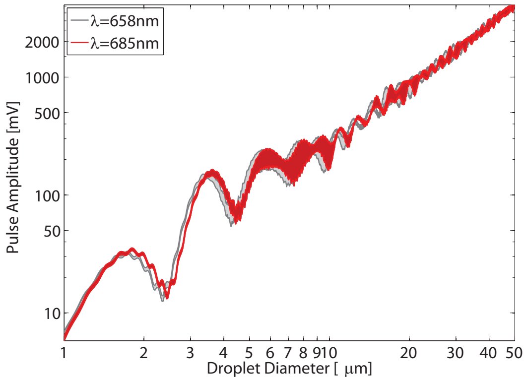
Figure 1: Mie band for laser wavelength \lambda = 658 \text{ nm} and \lambda = 685 \text{ nm}
