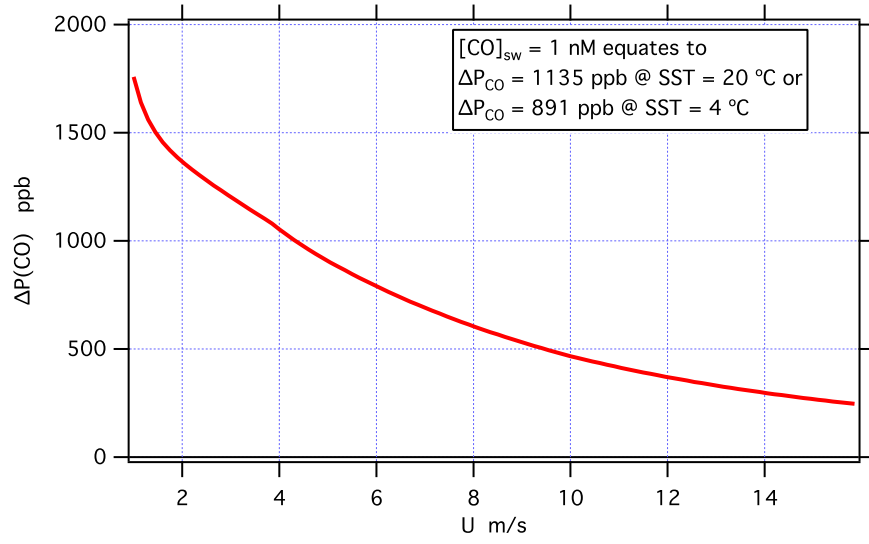
FIGURE 1. Air-sea concentration difference (expressed as \Delta P_{CO} ppb) for \delta F/F = 1 (100% error) in observed CO flux versus wind speed for a 1 hr sampling time under ideal stationary conditions.
