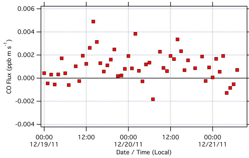
FIGURE 1. Hourly CO flux computed as the mean of 10-minute flux measurements selected for relative wind direction and stationarity criteria.
