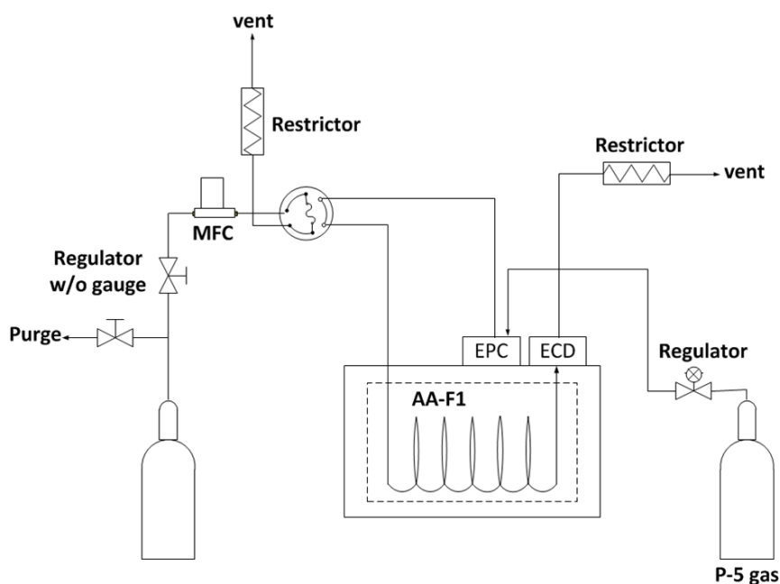
Fig. S1 Schematic diagram of the experimental setup
