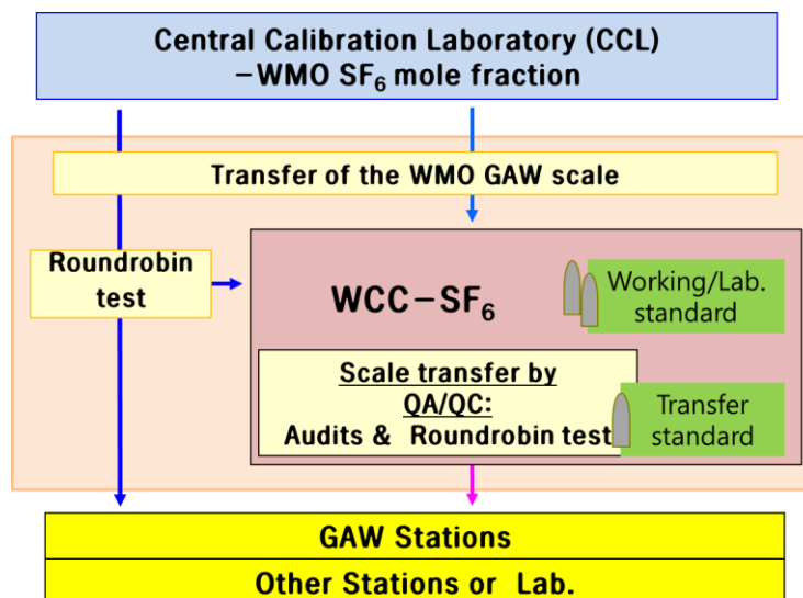
Fig. S2 Traceability chain of SF 6 through the CCL and GAW stations
