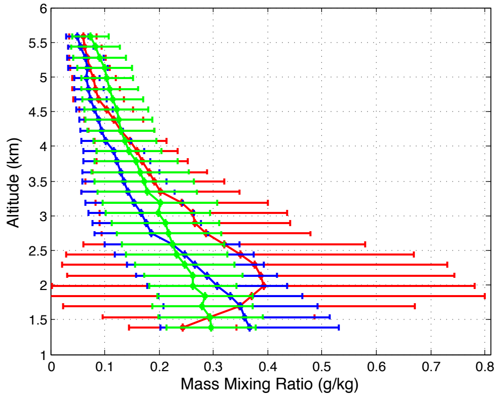
Fig. 7. Yearly variability of water vapour mixing ratio during polar sunrise (February to March) for 2007 (red), 2008 (blue) and 2009 (green). The horizontal bars are the root-mean square deviation of the measurement average for the measurement period. The water vapour variability was considerably larger in 2007 compared to the other two years.
