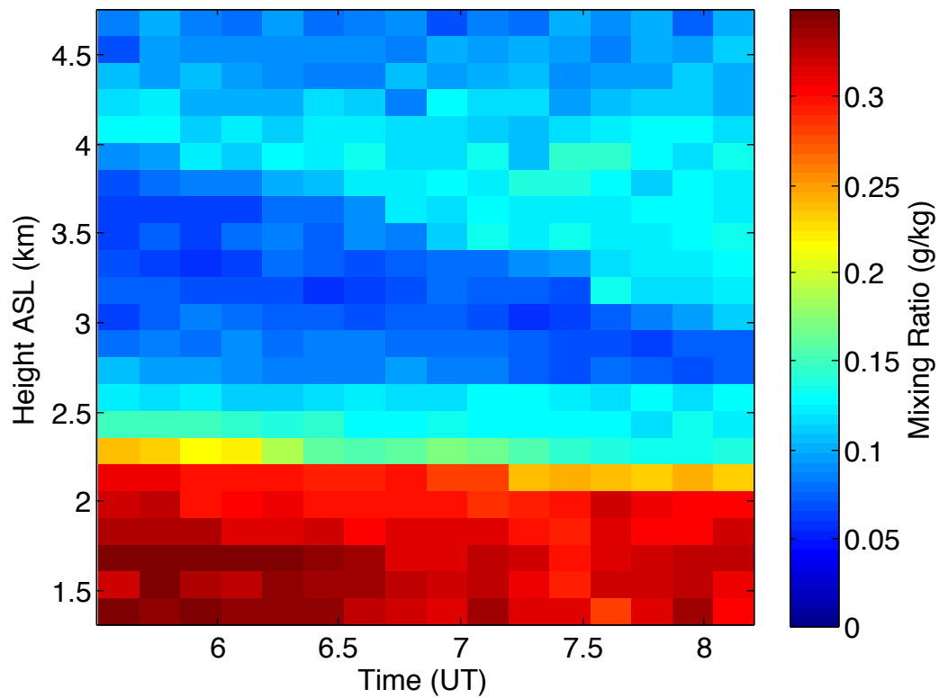
Fig. 8. Contour plot at a spatial resolution of 150 m and a temporal resolution of 10 min for measurements on the night of February 28, 2008. This night was chosen as an example of period of relatively small changes in water vapour mixing ratio compared to most of the other 39 nights available. However, even on this night the water vapour increases 25 to 50% above 3 km altitude.
