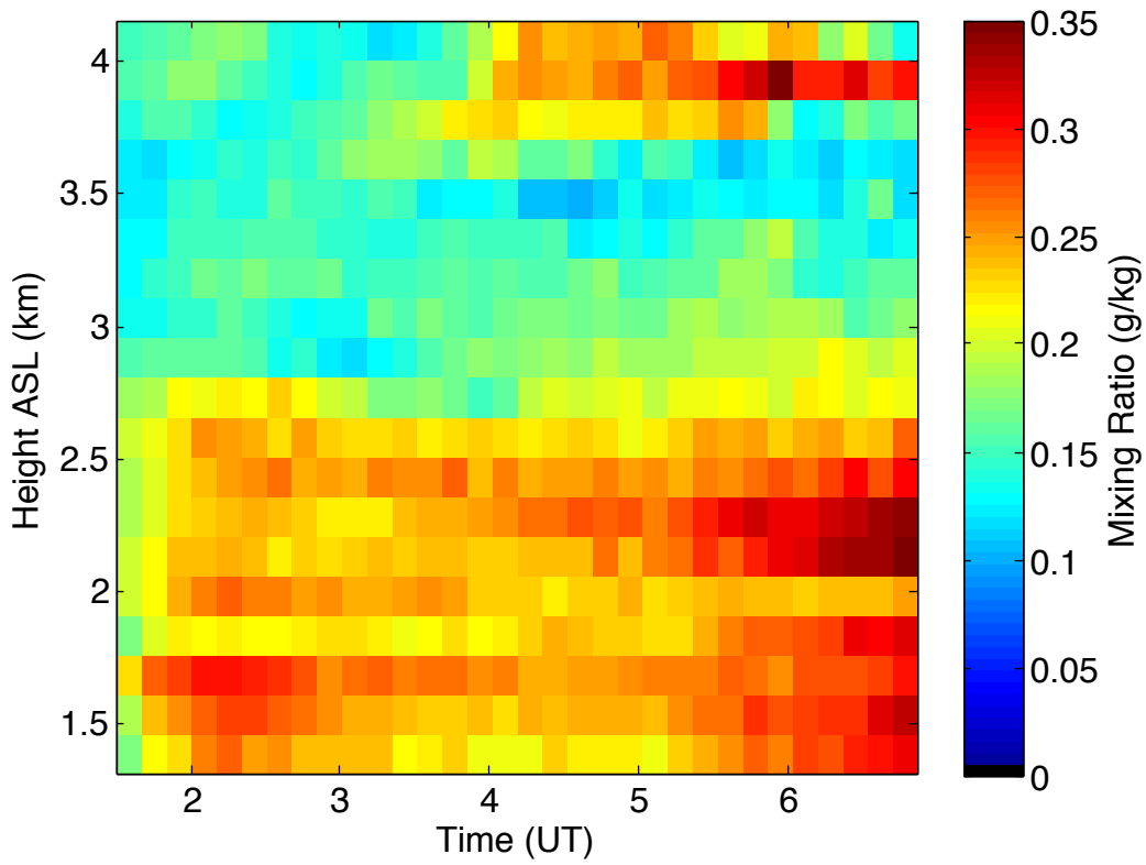
Fig. 9. Contour plot at a spatial resolution of 150 m and a temporal resolution of 10 min for measurements on the night of February 18, 2007. This night was chosen as an example of period with a rapid increase in the water vapour mixing ratio after 0400 UT.
