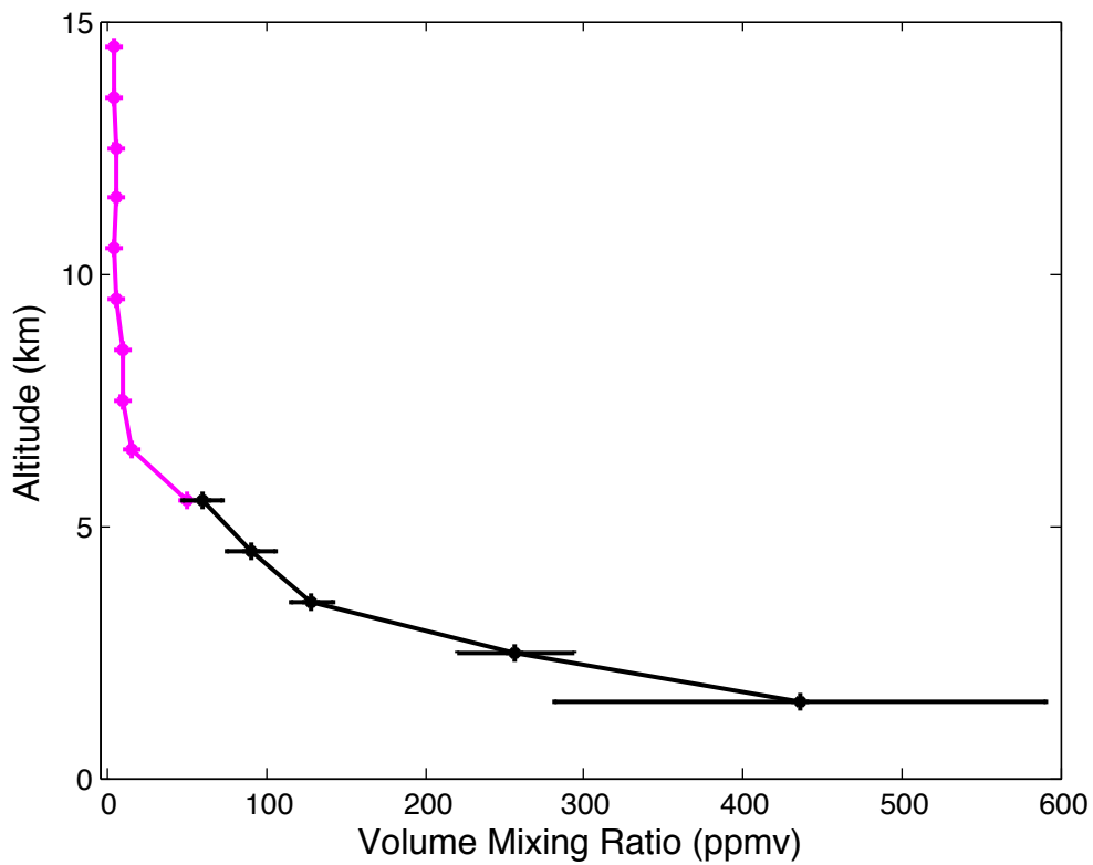
Fig. 6. Comparison of water vapour mixing ratio measurements made by the CEC-Lidar (black) and ACE-FTS (magenta). The lidar profile is the average from 0340 to 0850 UT on the night of February 28 2008. The ACE-FTS profile is for measurements taken at 2040 UT near Eureka on February 27 2008.
