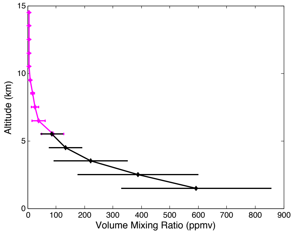
Fig. 5. Comparison of water vapour mixing ratio measurements made by the CEC Lidar (black) and ACE-FTS (magenta) in 2008. The ACE-FTS profile is the average of all measurements within 200 km (measured from the 30 km point of the ACE-FTS occultation and the CEC-Lidar) made during the Canadian Arctic ACE Validation Campaign period. The lidar profile is the average of the coincident nights. The horizontal bars indicate the RMS deviation of the average.
