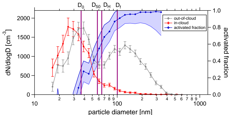
Fig. 3. Average number size distribution of total aerosol particles (grey crosses; out-of-cloud) and of interstitial aerosol particles (red crosses; in-cloud). The error bars correspond to the individual standard errors calculated as described in Sect. 2.4. The activated fraction (blue line; grey minus red, divided by grey; shaded area is the range of the statistical error of the data points) is plotted on the right axis. To assure comparability of the size distributions their averaging times were chosen to be unambiguous with respect to LWC for in-cloud (mean LWC = 0.131 \text{ gm}^{-3} ) and out-of-cloud conditions (mean LWC = 0.016 \text{ gm}^{-3} ) within a short time interval (in-cloud: 19 September 2012 15:00–16:00 UTC; out-of-cloud: 19 September 2012 17:30–18:00 UTC). The vertical lines indicate the diameters of zero activation ( D_0 ), 50 % activation ( D_{50} ), Hoppel minimum ( D_H ), and full activation ( D_f ).
