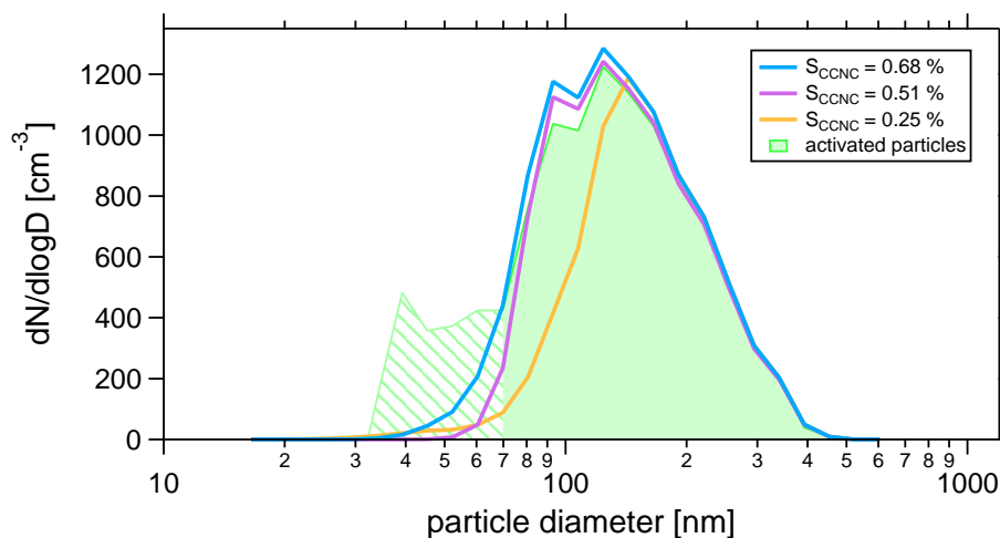
Fig. 4. Average number size distribution of activated particles in the cloud (green shaded area; hatched shoulder excluded from analysis) and CCN size distributions at S_{\text{CCNC}} = 0.25\% , 0.51\% , and 0.68\% (colored lines).
