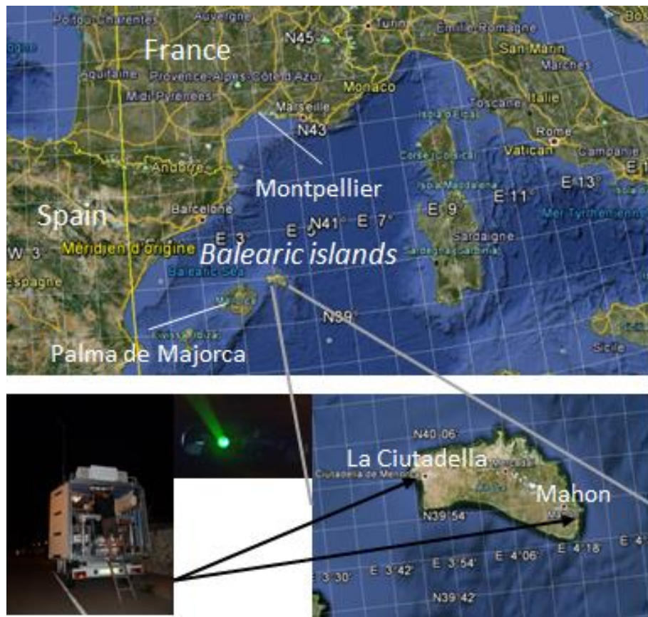
Fig. 3. Southern experimental sites selected for both the HyMeX/IODA-MED and the ChArMEx campaigns. The ground-based lidar-van is shown on the bottom-left. The main experimental sites are indicated on the map (courtesy of Google Inc.).
