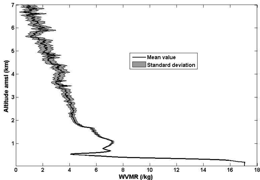
Fig. 10. WALI derived-WVMR profile (black) and its associated standard deviation (gray) averaged over 20 min (20000 laser shots) during the night of 19 October 2012 over Menorca.
